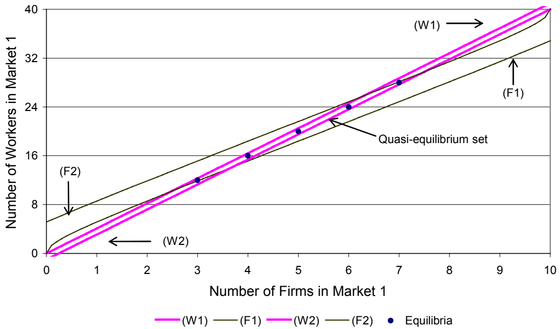
Figure II The Quasi-equilibrium Set in the Labor Market Model: F=10 , L=40 , \sigma = 1 , and \delta = 0.25 .
