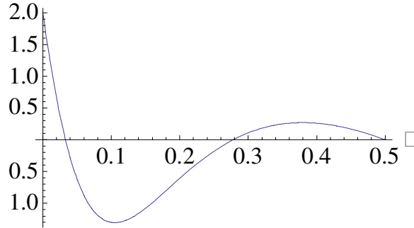
Advantage of Phase 1 Deviation
