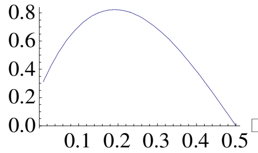
Advantage of Phase 1 Deviation, b \ll c \ll 2.5
