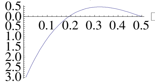
Advantage of Phase 1 Deviation, b \ll c \ll 4
