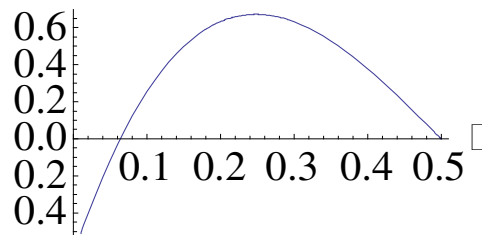
Advantage of Phase 1 Deviation, b \ll c \ll 4
