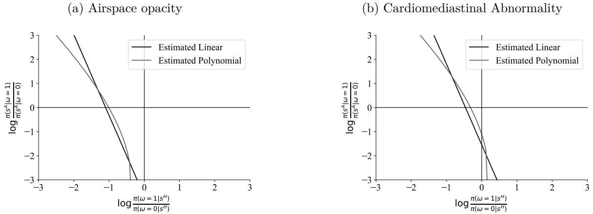
Figure C.10: Linearity of the Update Function
