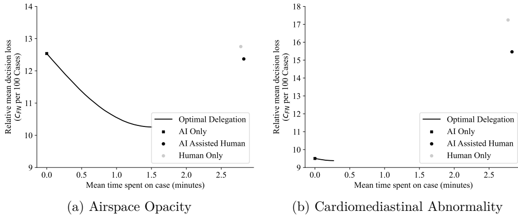
Figure C.15: Loss-time frontier: Heterogeneous human time cost
