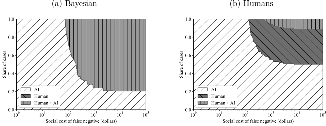
Figure C.16: Airspace Opacity modality shares with heterogeneous time cost
