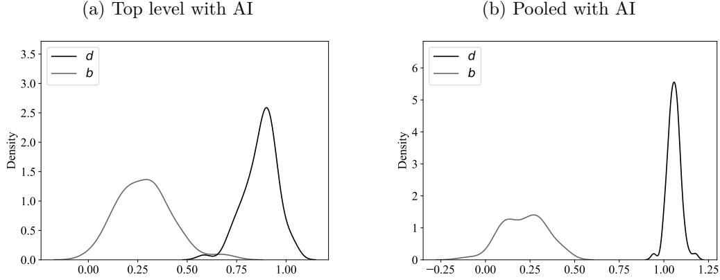
Figure C.11: Individual heterogeneity in b and d
