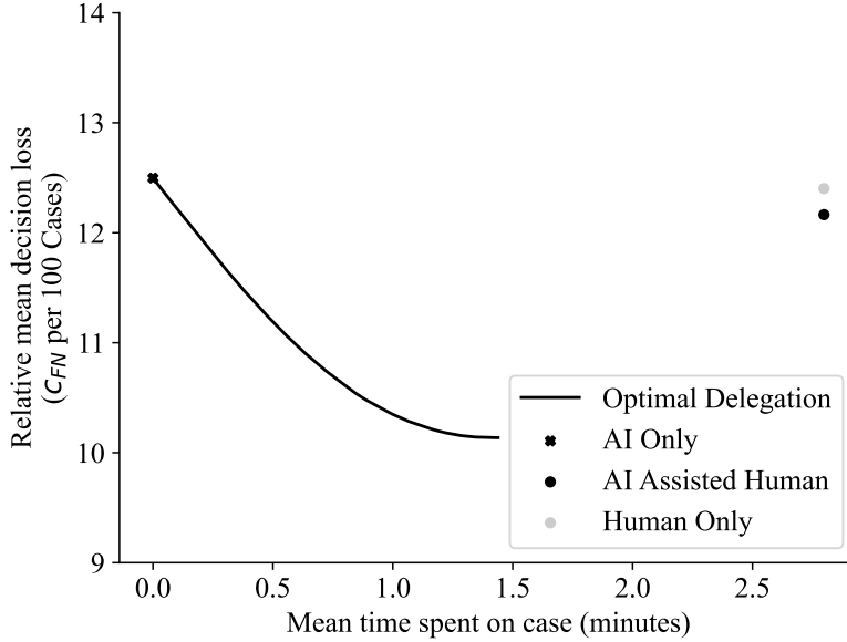
Figure 9: Loss-time frontier
