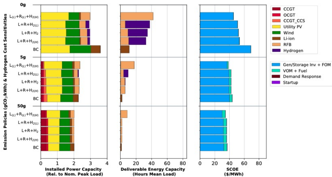
Figure 6.12: Impacts of low-, mid-, and high-cost hydrogen on installed power capacity, storage capacity, and SCOE, across a range of CO 2 constraints for the Texas region. They are, in ascending order: (1) base case (i.e., mid-cost Li-ion only, BC); (2-4) mid-cost Li-ion and RFB + incremental additions of high-cost hydrogen (L+R+H 2H ), mid-cost hydrogen (L+R+H 2 ), and low-cost hydrogen (L+R+H 2L ); and (5) low-cost Li-ion and RFB + high-cost hydrogen (L L +R L +H 2H ). Low-, mid-, and high-cost assumptions for each storage technology are defined in Table 6.3.
