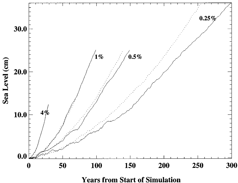
Figure 13. Global mean sea level rise due to thermal expansion caused by a 4%, 1%, 0.5%, and 0.25% per year increase in \text{CO}_2 in the simulations with the 2D-LO model with a sensitivity of 3.7^\circ\text{C} and K_v = 5.0 \text{ cm}^2/\text{s} (solid curves) and the GFDL GCM (dashed curves, R. Stouffer, private communication, 1996).
