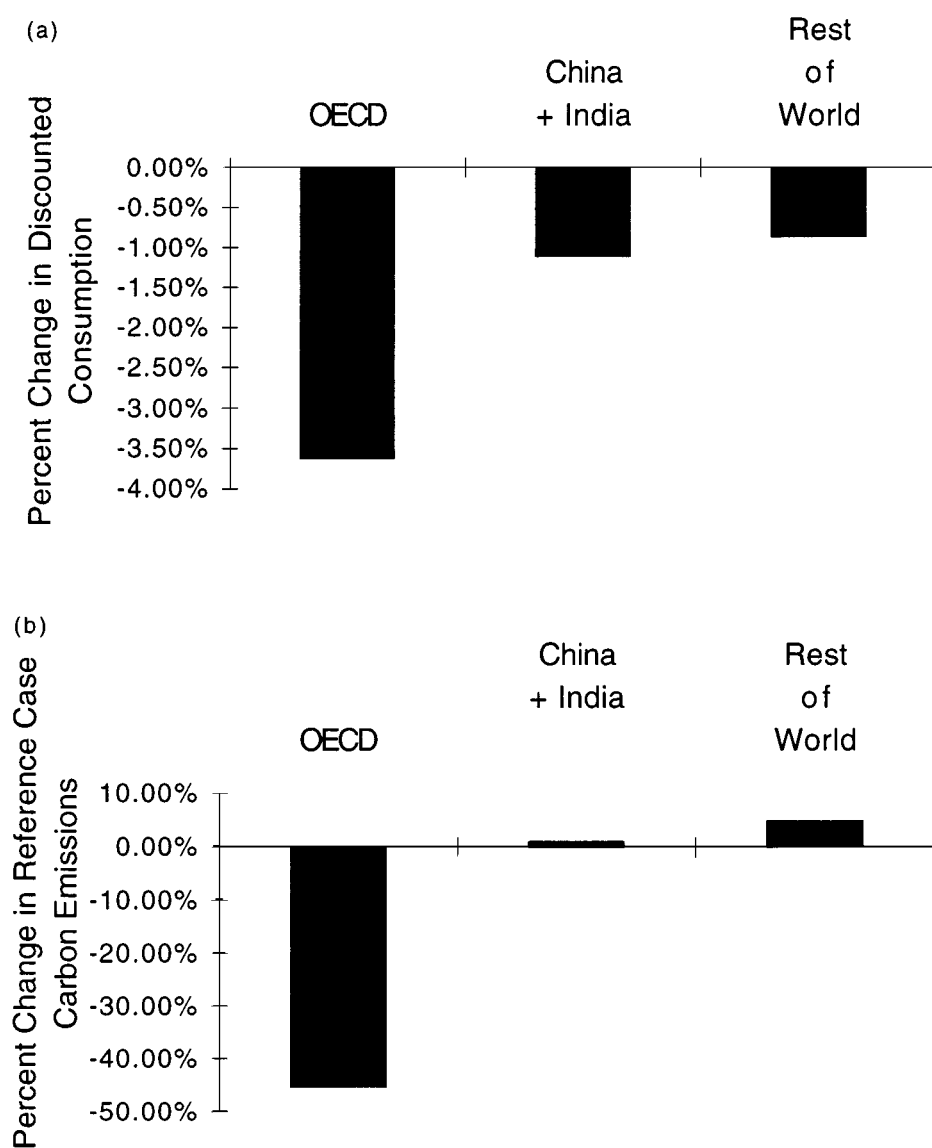
Figure 5. (a) Regional economic impacts of a version of the AOSIS Protocol (impacts expressed as the cumulative percentage loss in consumption between 2000 and 2100, discounted at 5% as computed from the differences between two appropriate runs of EPPA). (b) Percentage change in carbon emissions between 1990 and 2100 due to substitution effects and GDP loss resulting from AOSIS Protocol, as computed from the differences between two appropriate runs of EPPA. See Figure 4 for regional abbreviations.
