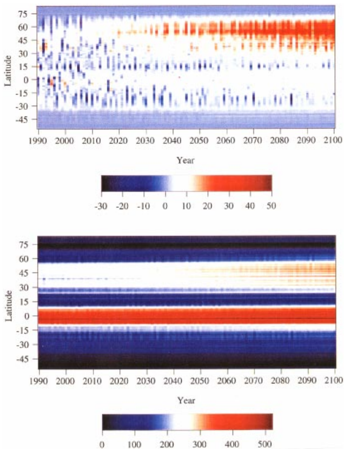
Figure 21. Longitudinally cumulative terrestrial NEP (upper panel) and NPP (lower panel) predicted as a function of latitude (in degrees with positive denoting North and negative denoting South) and time (in years) in the transient TEM reference run. Units are TgC/yr (MtC/yr) for each 0.5 degree latitude band.
