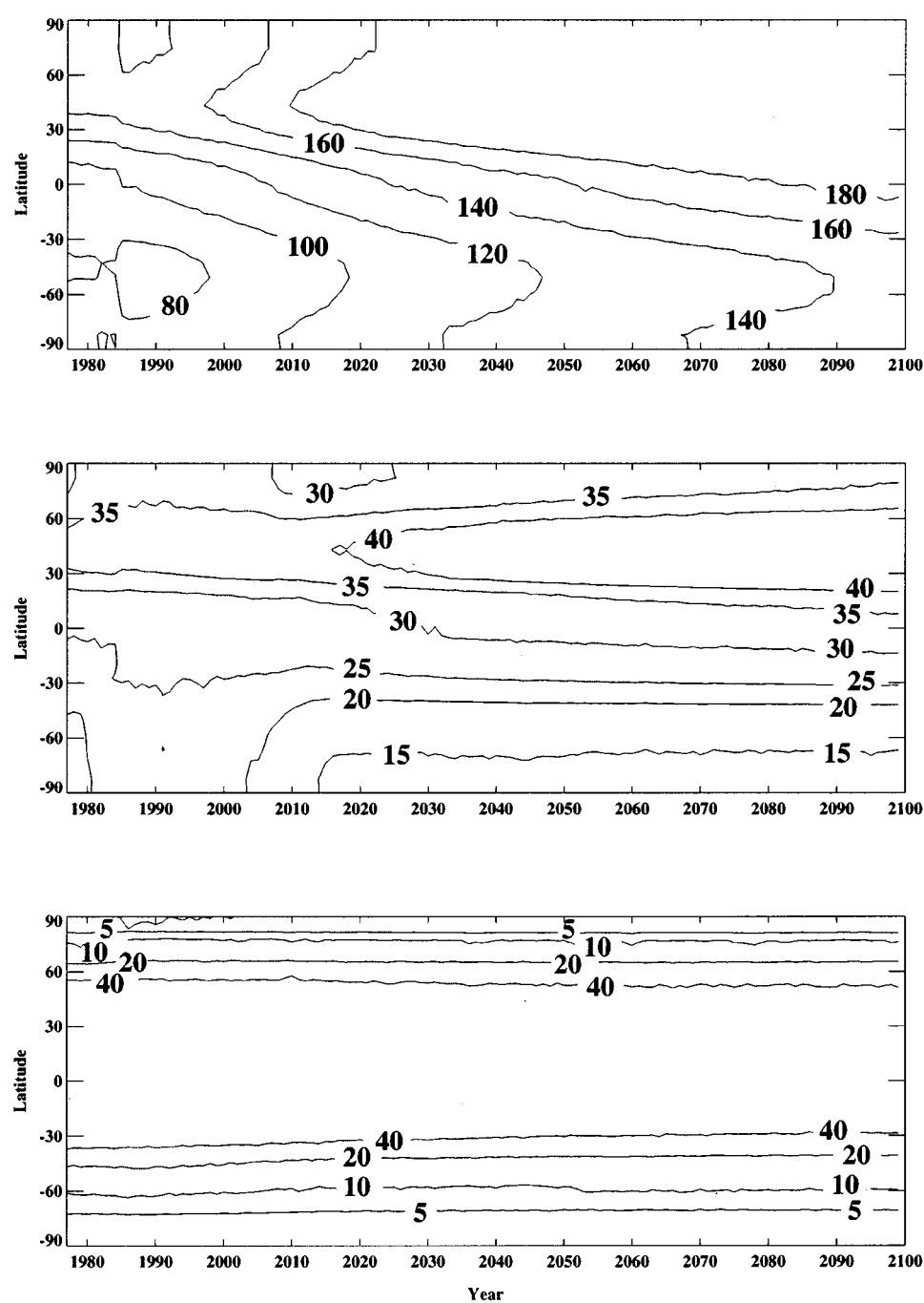
Figure 17. Temporal evolution of the annual-mean surface air concentrations of CO (upper panel, in ppb), O 3 (middle panel, in ppb), and OH (lower panel, 10^{-3} ppt) as functions of latitude (in degrees, denoted as positive in Northern Hemisphere, negative in Southern Hemisphere) in the reference run.
