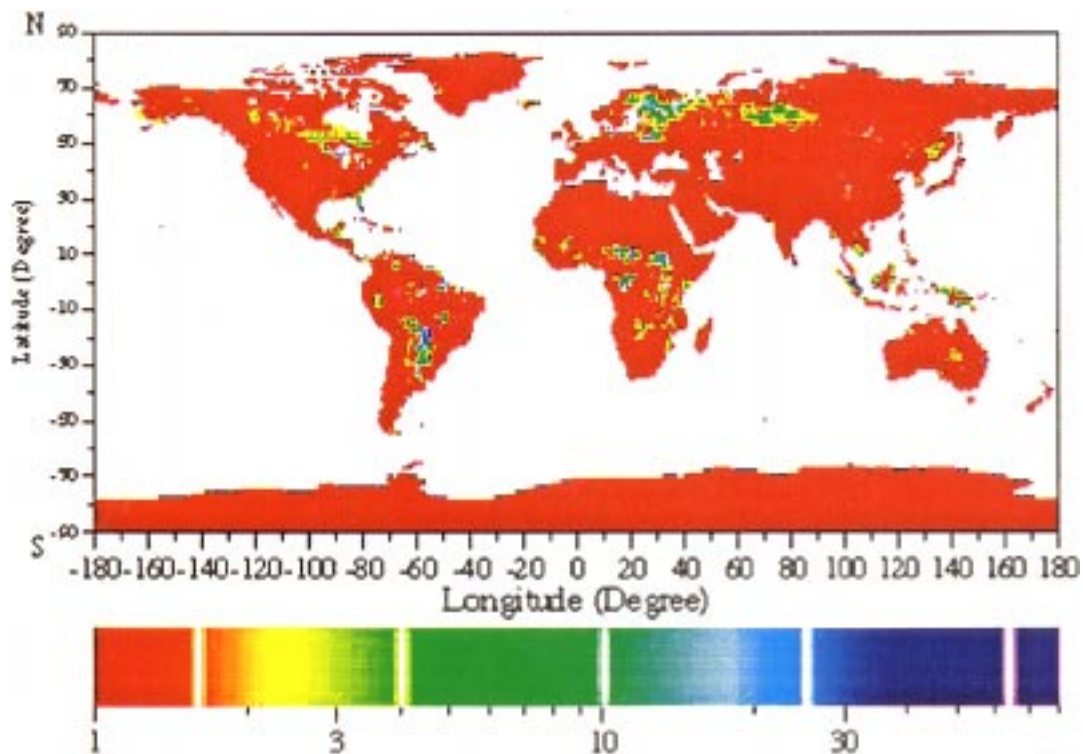
Figure 7. Predicted annual-average wetland \text{CH}_4 emissions ( 10^9 \text{ g CH}_4/\text{degree}^2/\text{month} ) from Natural Emissions Model at 1^\circ \times 1^\circ resolution.
