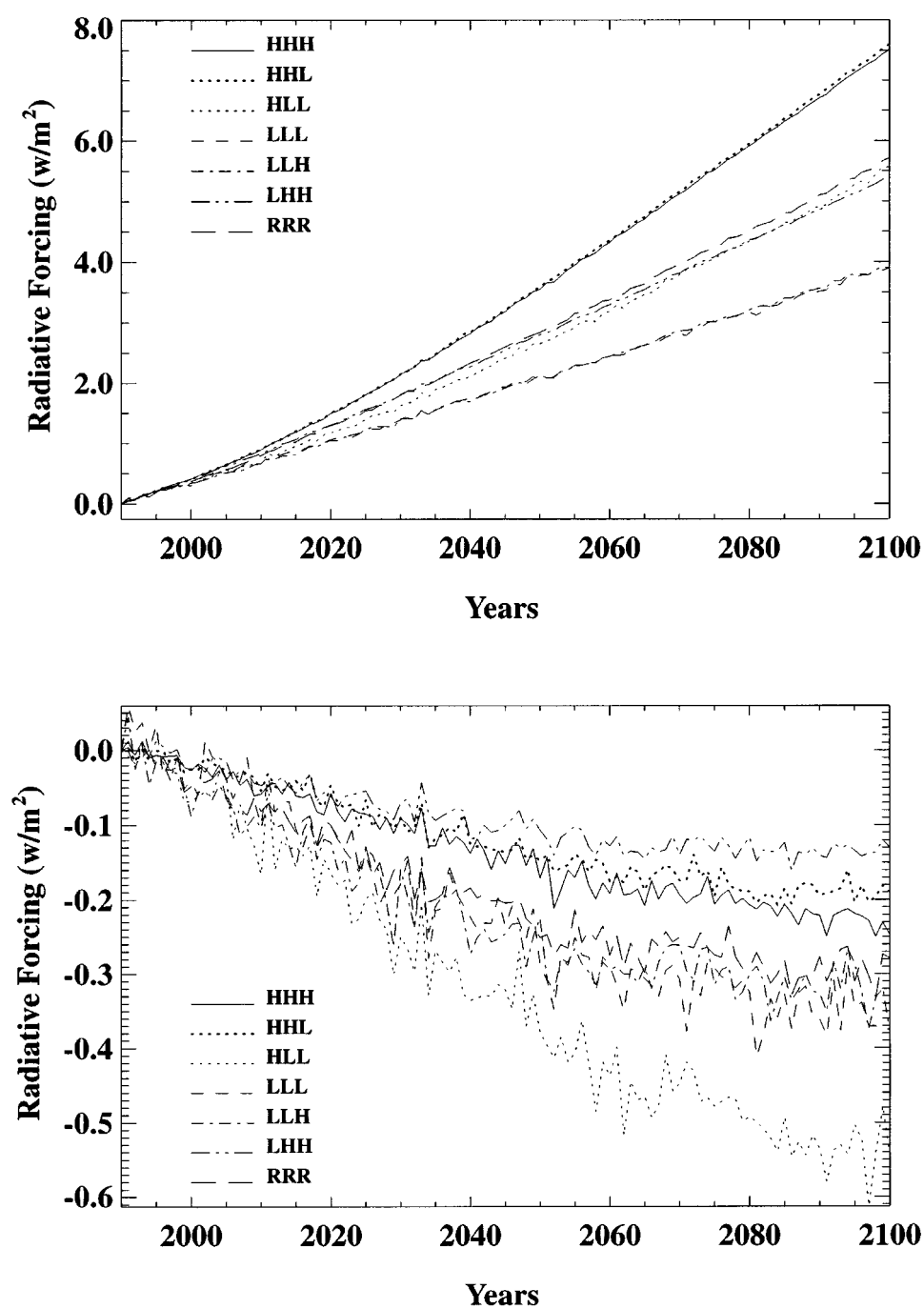
Figure 27. Predicted changes in radiative forcing (exclusive of H 2 O) from 1990 levels (W/m 2 ) in the seven sensitivity runs. The upper set of curves refers to all gases and aerosols and the lower set to aerosols alone. See Figure 23 for run nomenclature.
