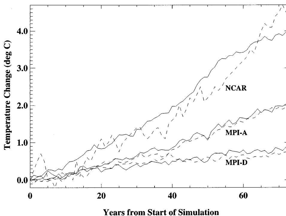
Figure 12. Global mean surface air temperature change caused by prescribed increases in CO 2 in the simulations with the MPI and NCAR GCMs (dashed curves) and in the matching versions of the 2D-LO model (solid curves). Prescribed increases are 1% per year for the NCAR model and IPCC IS92(A) and (D) for the MPI model.
