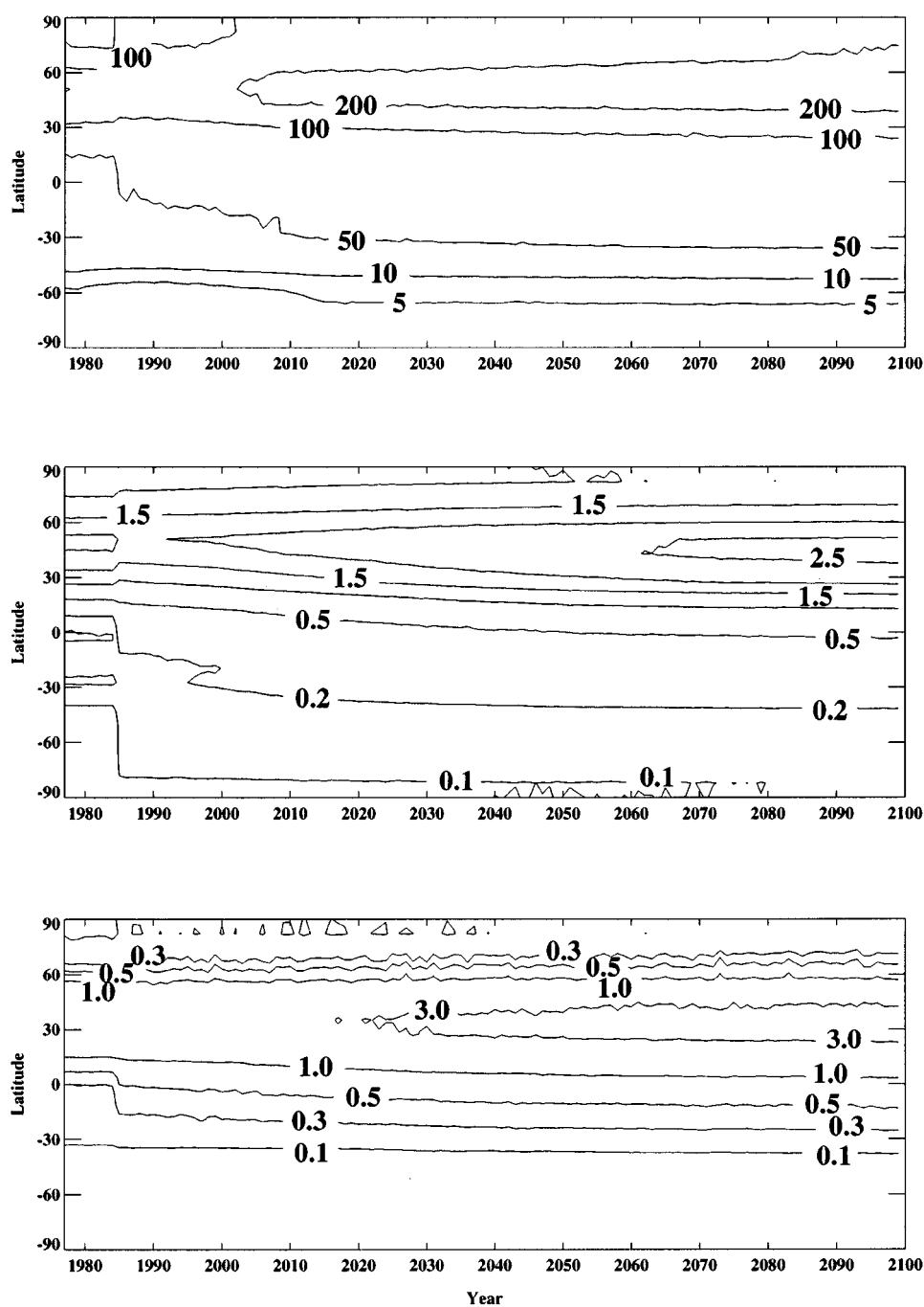
Figure 18. As in Figure 17, but for \text{NO}_x (upper panel, in ppt), anthropogenic \text{SO}_2 (middle panel, in ppb), and \text{H}_2\text{SO}_4 vertical optical depth (lower panel, actual dimensionless values are multiplied by 100 for display here).
