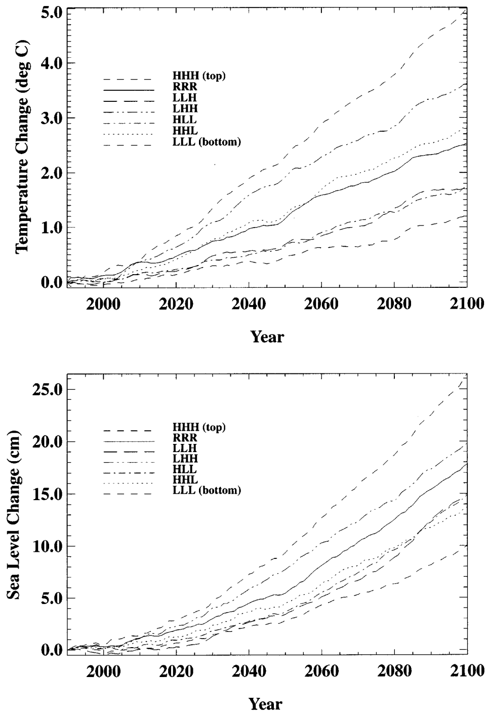
Figure 29. Changes in global-average surface air temperatures (upper panel, °C) and sea-level (lower panel, cm of rise due to ocean thermal expansion only) from 1990 values in the seven sensitivity runs.
