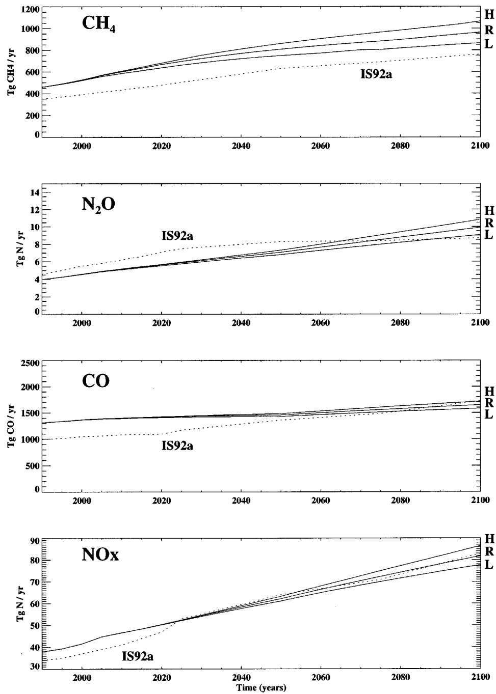
Figure 25. As for Figure 24 but for emissions of CH 4 (TgCH 4 /yr), N 2 O (TgN/yr), CO (TgCO/yr), and NO x (TgN/yr). See Figure 23 for run nomenclature.
