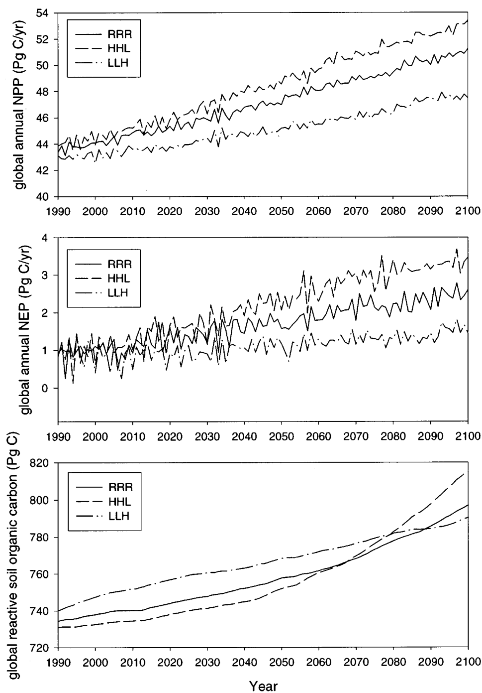
Figure 32. Global NPP (upper panel), NEP (middle panel), and reactive soil organic carbon (lower panel) predicted in transient TEM driven by the CO 2 and climate variables from the reference and two selected sensitivity runs.
