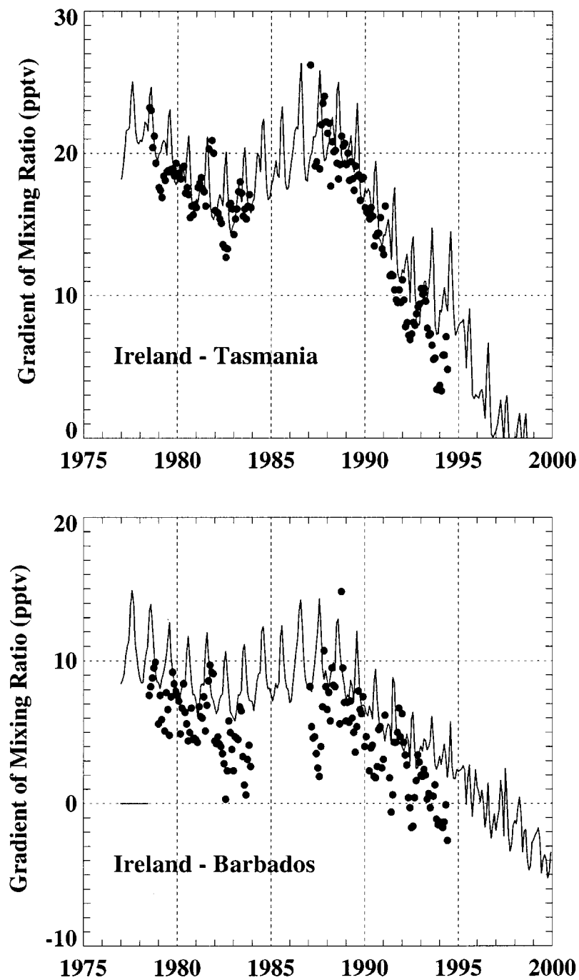
Figure 8. Time evolution of the latitudinal gradient of surface \text{CFC}_{13} mixing ratio, defined as the differences between mixing ratios at Ireland ( 52^\circ \text{N} ) and Tasmania ( 40^\circ \text{S} ) [upper graph], and between mixing ratios at Ireland and Barbados ( 13^\circ \text{N} ) [lower graph], for the model (solid lines) and observations (dots).
