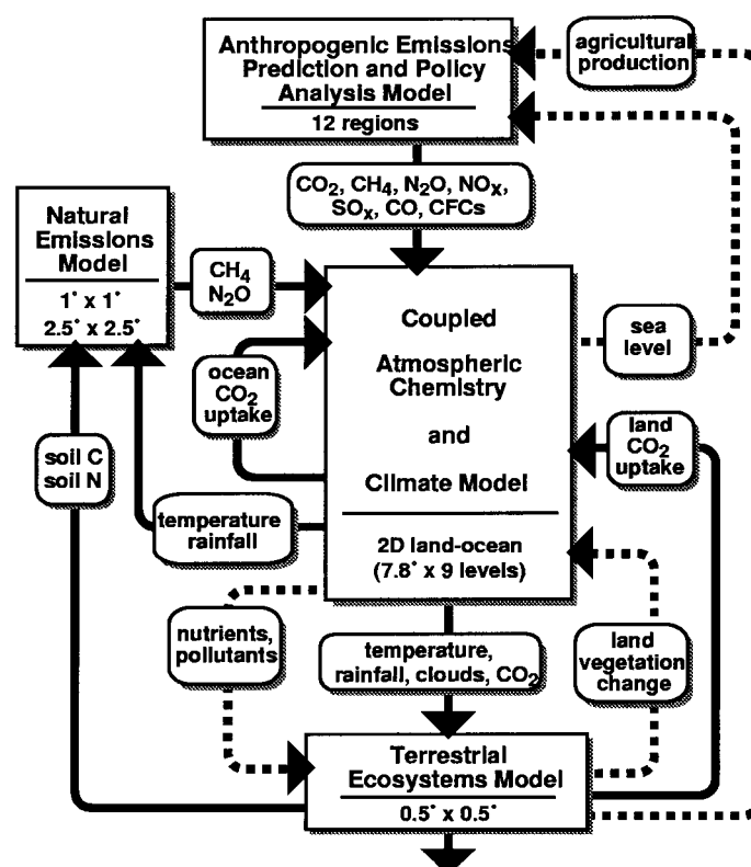
Figure 1. Schematic illustrating the framework and components of the MIT global system model. Feedbacks between the component models which are currently included or under development for future inclusion are shown as solid and dashed lines, respectively.
