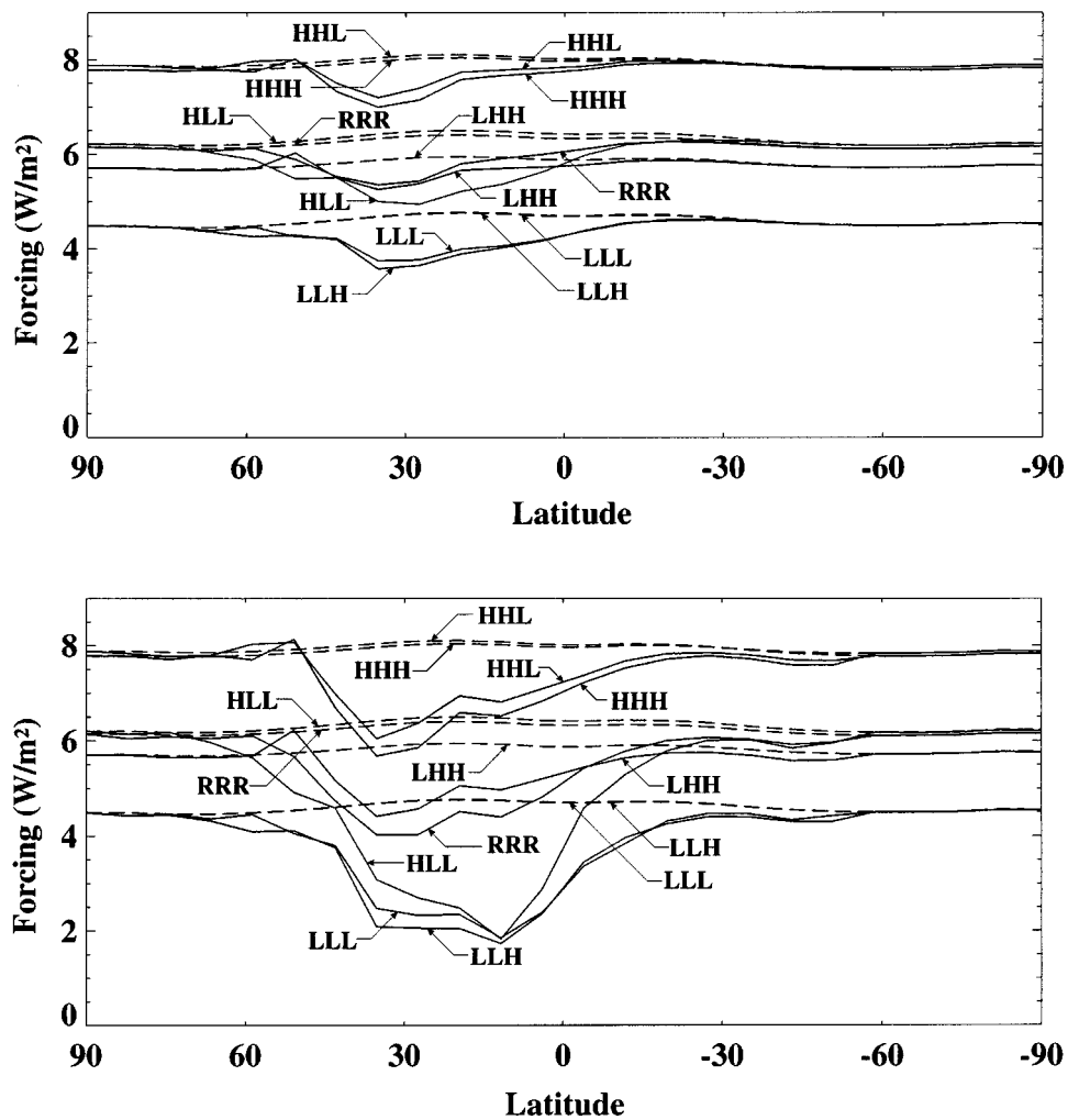
Figure 28. Predicted changes (between 1990 and the average for 2090–2100) in total radiative forcing (solid lines) and forcing due to gases only (dashed lines) for the seven sensitivity runs. Upper panel refers to longitudinal averages over land plus ocean and lower panel over land alone. Units are \text{W/m}^2 .
