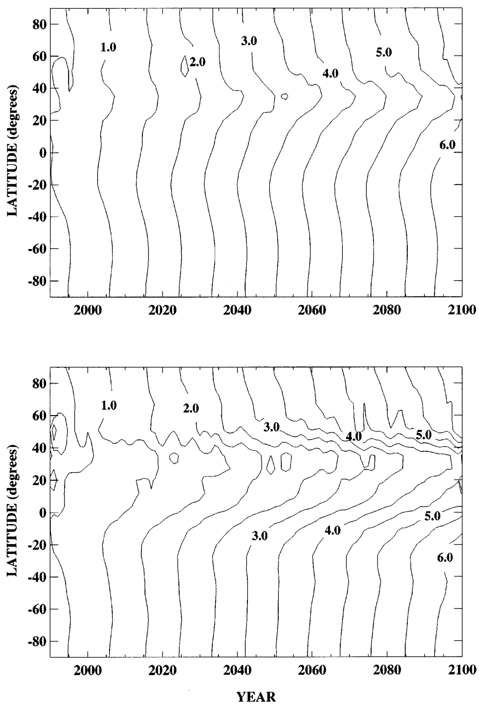
Figure 19. Changes in longitudinally averaged radiative forcing ( \text{watt/m}^2 ) from 1990 levels for land and ocean (upper panel), and land only (lower panel), are given as functions of latitude (in degrees, with positive values in Northern Hemisphere and negative values in Southern Hemisphere) and time (in years).
