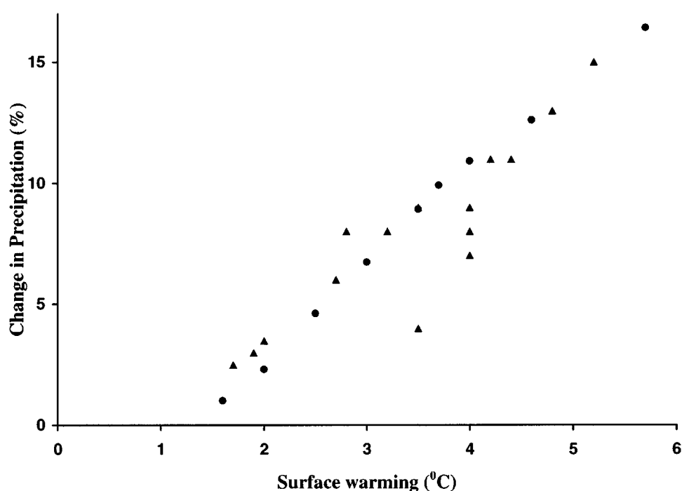
Figure 10. Percentage change in globally and annually averaged precipitation as a function of equilibrium global mean surface warming caused by a doubling of \text{CO}_2 as predicted by different GCMs (triangles; from IPCC, 1990) and different versions of the 2D-LO model (circles).
