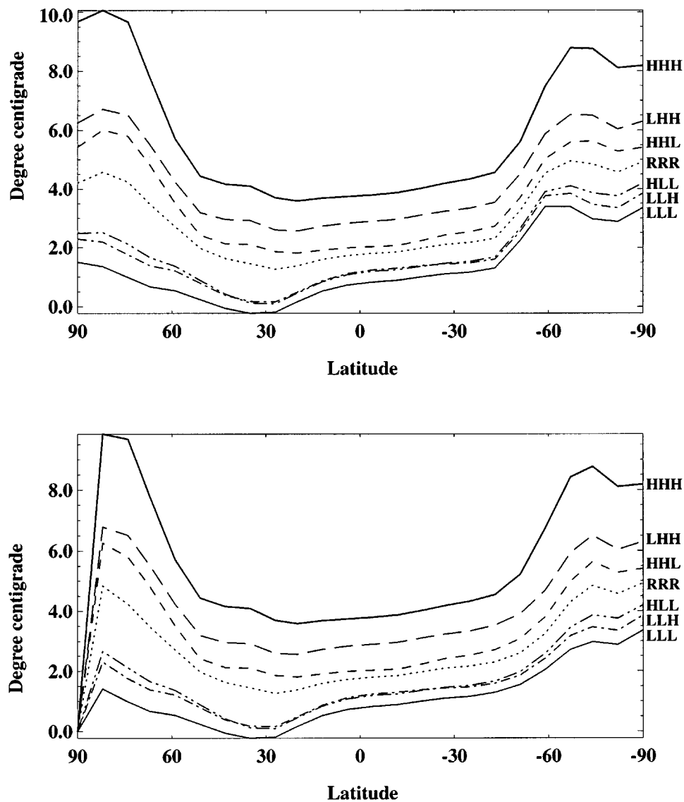
Figure 30. Changes (between 1990 and the average for 2090–2100) of longitudinally averaged surface air temperature ( ^{\circ}\text{C} ) over land plus ocean (upper panel) and land only (lower panel) for the seven sensitivity runs. Latitude in degrees, with positive values denoting Northern Hemisphere.
