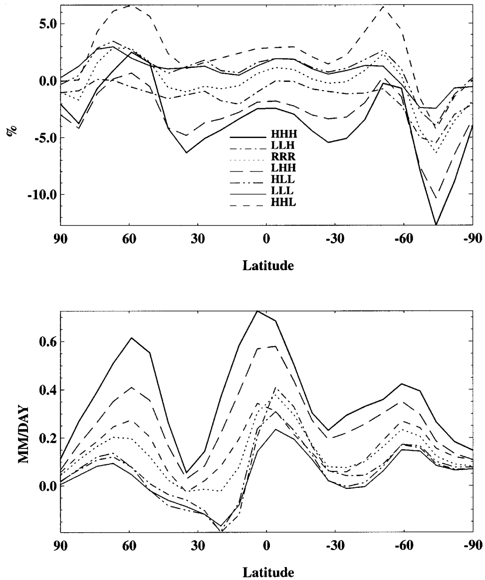
Figure 31. Changes (between 1990 and the average for 2090–2100) of longitudinally averaged cloud cover (upper panel, % cover) and precipitation (lower panel, mm/day) over land for the seven sensitivity runs. Latitude in degrees, with positive values denoting Northern Hemisphere.
