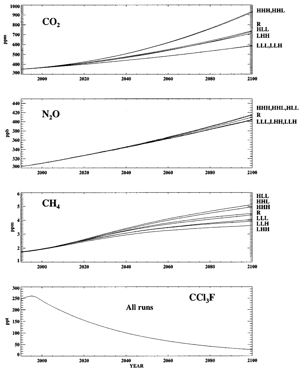
Figure 26. Predicted CO 2 (ppm), N 2 O (ppb), CH 4 (ppm); and CCl 3 F (ppt) mixing ratios for the seven sensitivity runs of the coupled chemistry/climate model. Emissions and hence mixing ratios of the chlorofluorocarbon CCl 3 F are the same in all seven runs. See Figure 23 for run nomenclature.
