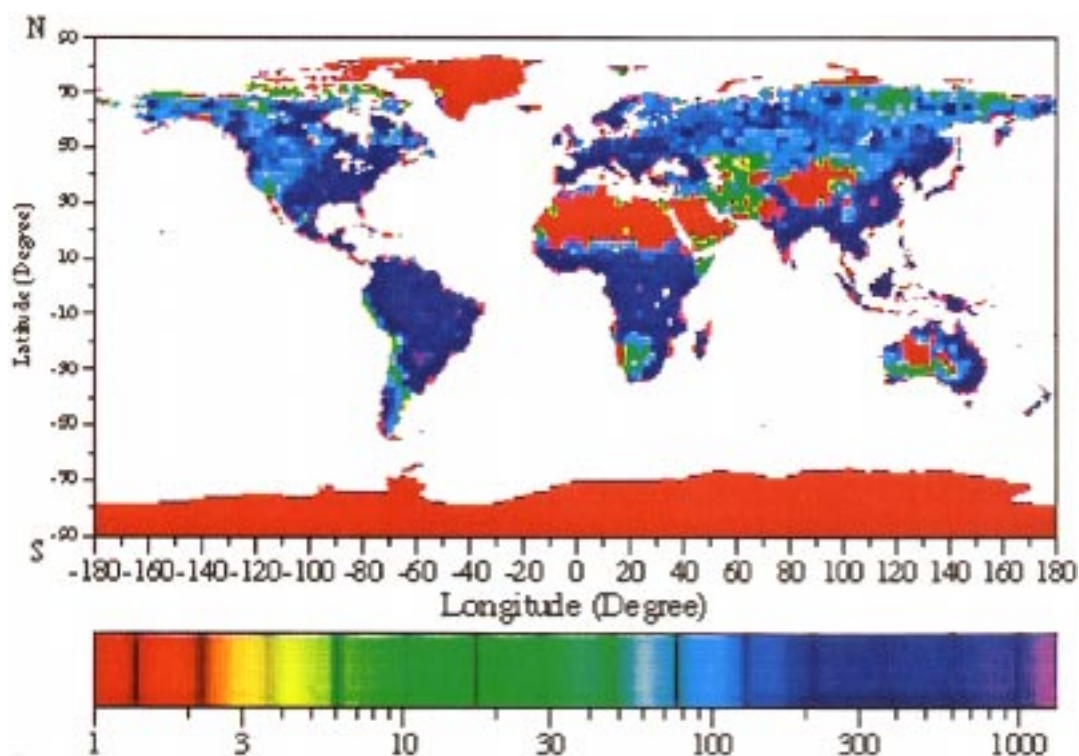
Figure 6. Predicted annual-average soil \text{N}_2\text{O} emissions ( \text{gN/hectare/month} ) from Natural Emissions Model at 2.5^\circ \times 2.5^\circ resolution.
