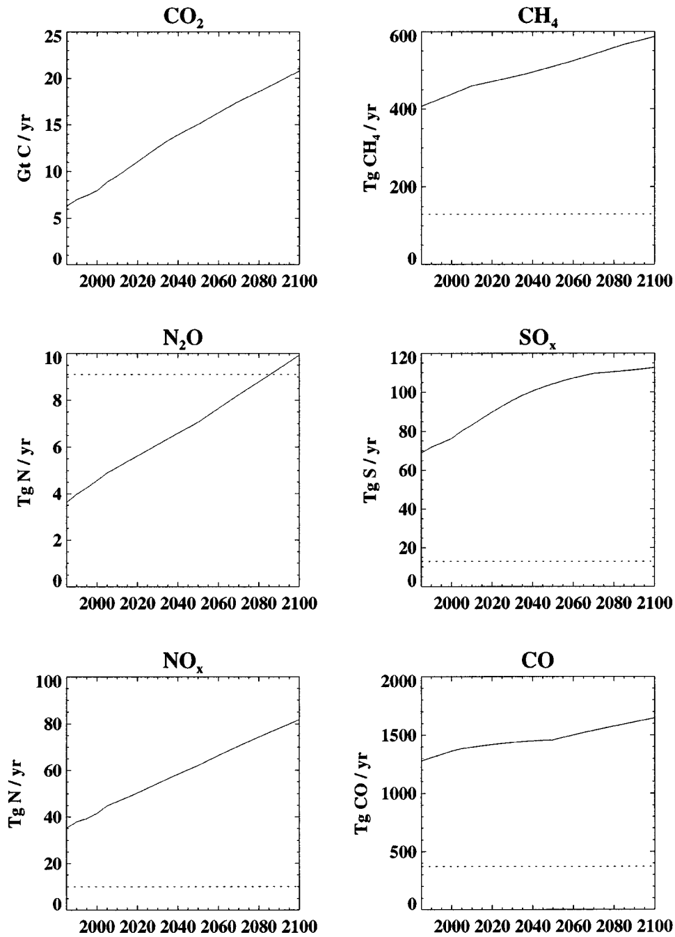
Figure 15. Annual EPPA (solid lines) and natural (dotted lines) emissions for the Reference Run.
