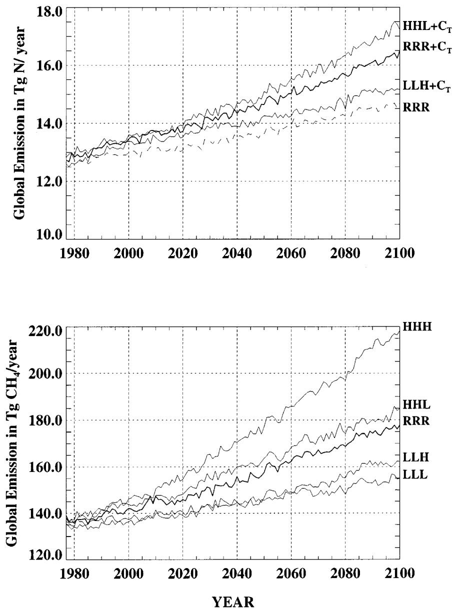
Figure 33. Predicted annual natural emissions of N 2 O (upper panel, TgN/year) and CH 4 (lower panel, TgCH 4 /year) in NEM runs driven by the indicated climate model runs and (for N 2 O) also by the indicated climate plus TEM model runs (the latter denoted by the addition of C T to the run designation).
