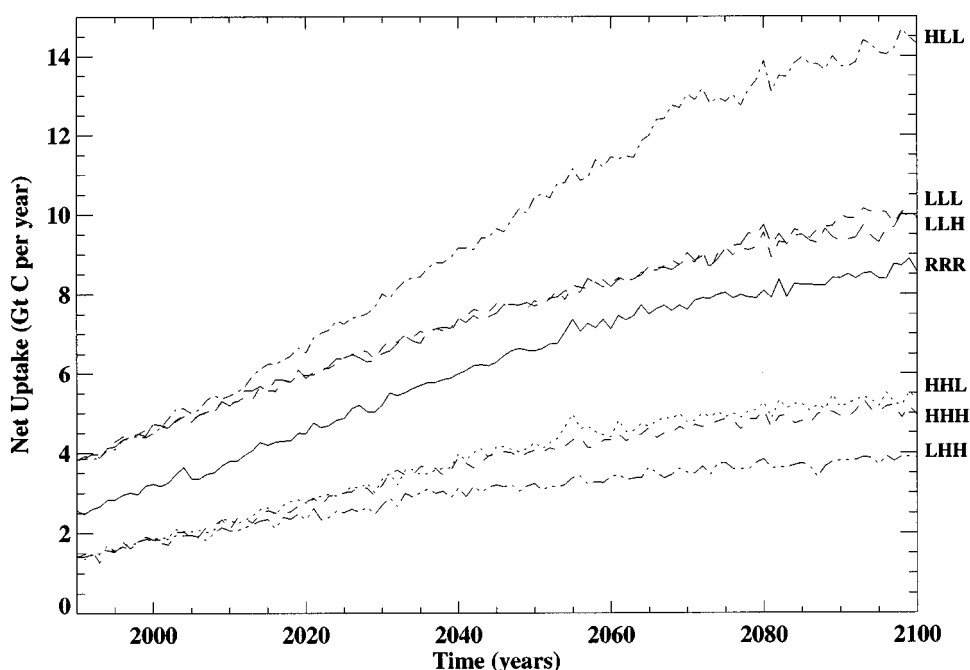
Figure 34. Predicted annual uptake rate of carbon (GtC/year) by the ocean predicted in the indicated OCM runs.
