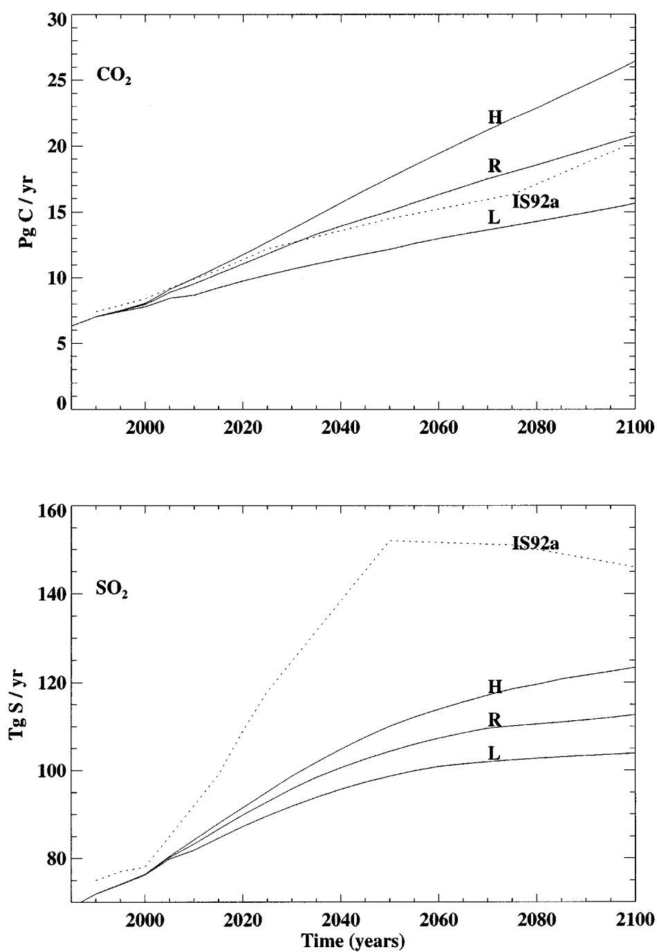
Figure 24. Higher (H), lower (L), and reference (R) CO 2 emissions (PgC/yr, GtC/yr) (upper graph) and SO 2 emissions (TgS/yr) (lower graph) from EPPA runs and IS92a IPCC (1992) emission scenarios. See Figure 23 for run nomenclature.
