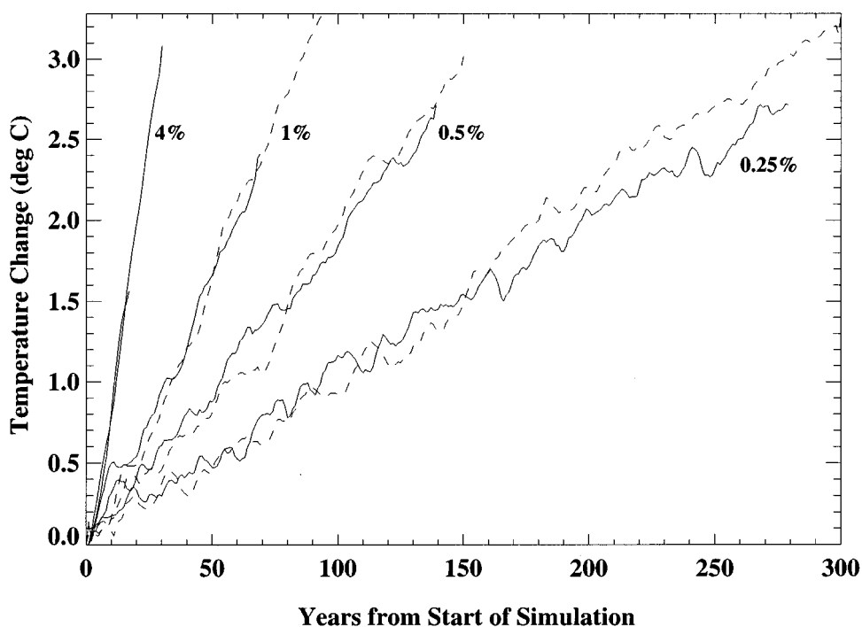
Figure 11. Global mean surface air temperature change caused by a 4%, 1%, 0.5%, and 0.25% per year increase in \text{CO}_2 in the simulations with the 2D-LO model with a sensitivity of 3.7^\circ\text{C} and K_v = 5.0 \text{ cm}^2/\text{s} (solid curves) and the GFDL GCM (dashed curves, R. Stouffer, private communication, 1996).
