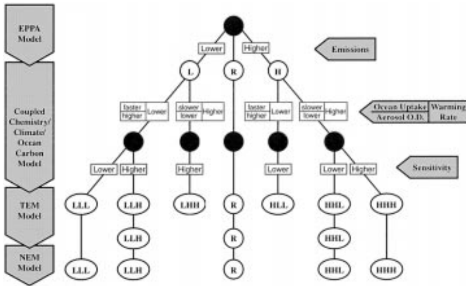
Figure 23. Schematic illustrating the runs performed for the sensitivity analysis of the IGSM. Open circles denote points in sequence where output is available, with the letters in the circle denoting the identifying symbol for the output.
