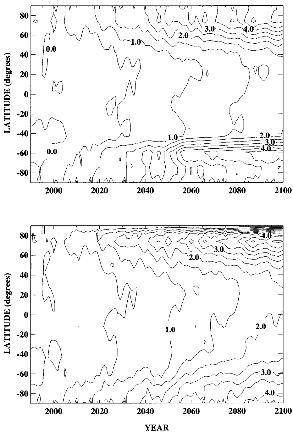
Figure 20. As in Figure 19 but for surface temperature change ( ^{\circ}\text{C} ) over land and ocean (upper panel) and over land only (lower panel).
