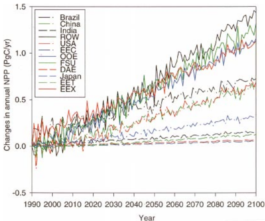
Figure 22. Predicted changes in NPP from their 1990 levels in the 12 EPPA economic regions as a function of time (in years) in the transient TEM reference run. Units are PgC/yr (GtC/yr).
