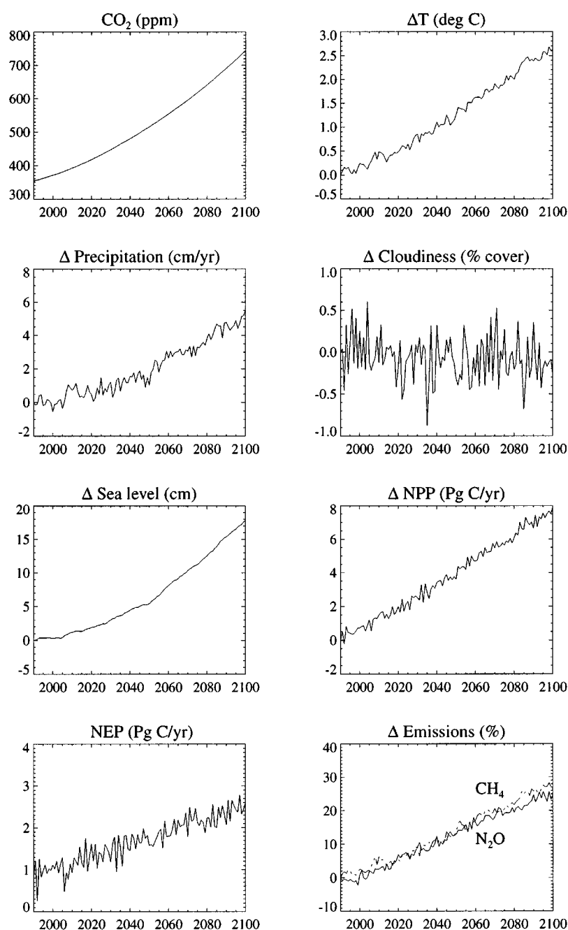
Figure 16. Predictions from the global system model for either the global-total or global-average values, or the changes ( \Delta ) in these values from their 1990 levels, are given for \text{CO}_2 concentrations, surface air temperature, precipitation, cloudiness, sea level, net primary production, net ecosystem production, and natural \text{N}_2\text{O} and \text{CH}_4 emissions as a function of time for the reference run.
