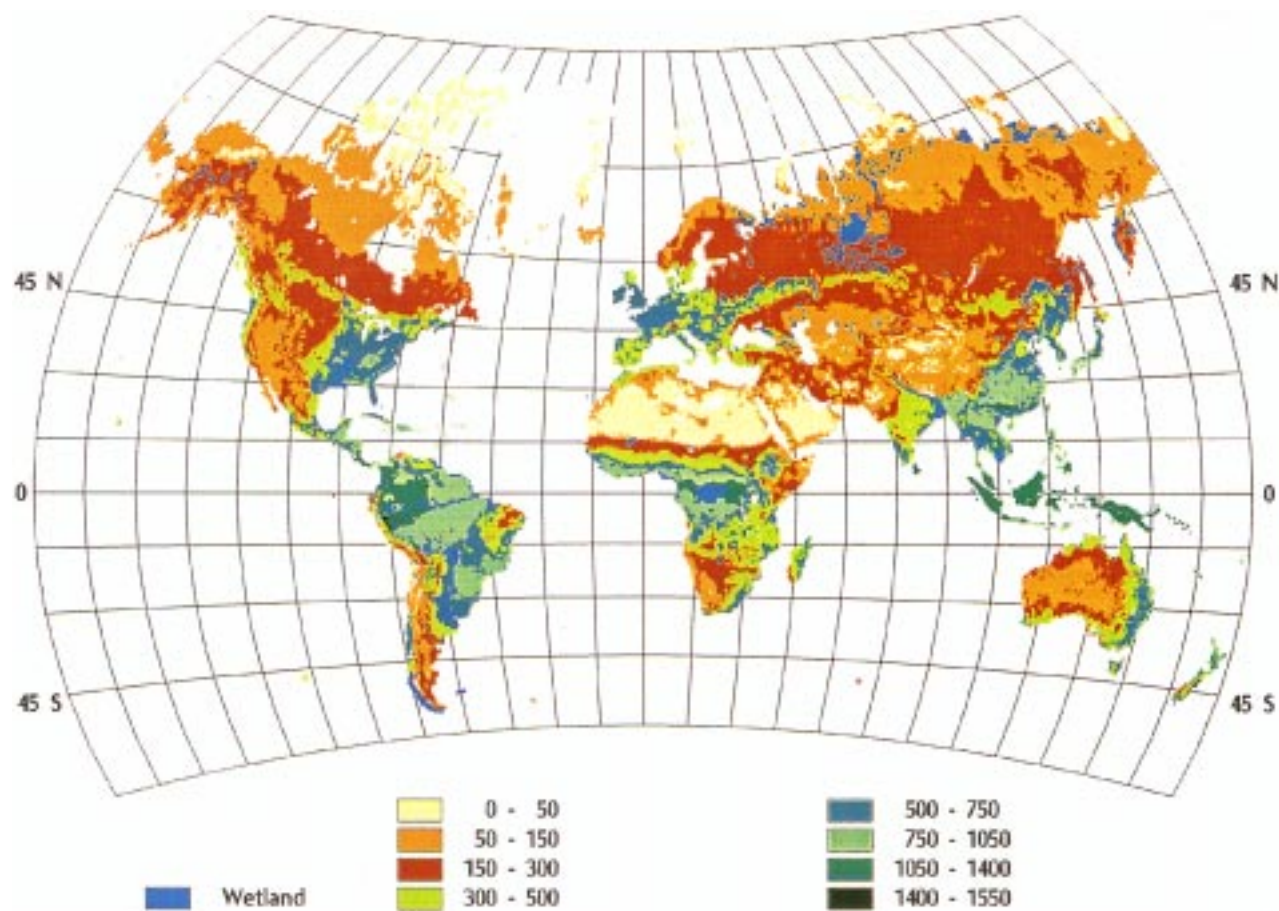
Figure 14. Estimates of Net Primary Production (NPP) (gC/m 2 /yr) for CO 2 levels of 315 ppm and contemporary climate defined by long-term mean climate data (Cramer and Leemans, 1993; W. Cramer, private comm.).
