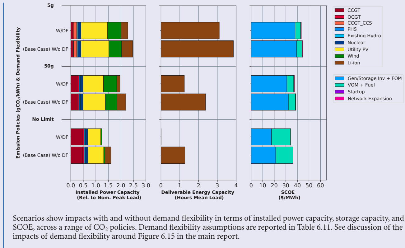
Figure C.11 System impacts of demand flexibility in the Southeast
