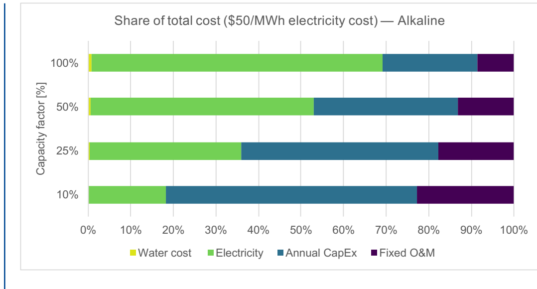
Figure 5.10 Cost breakdown by variable
