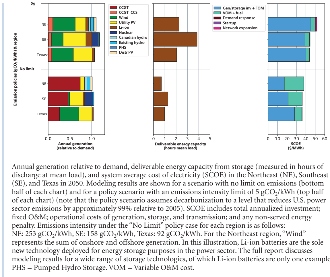
Figure ES.3: Annual generation relative to demand
