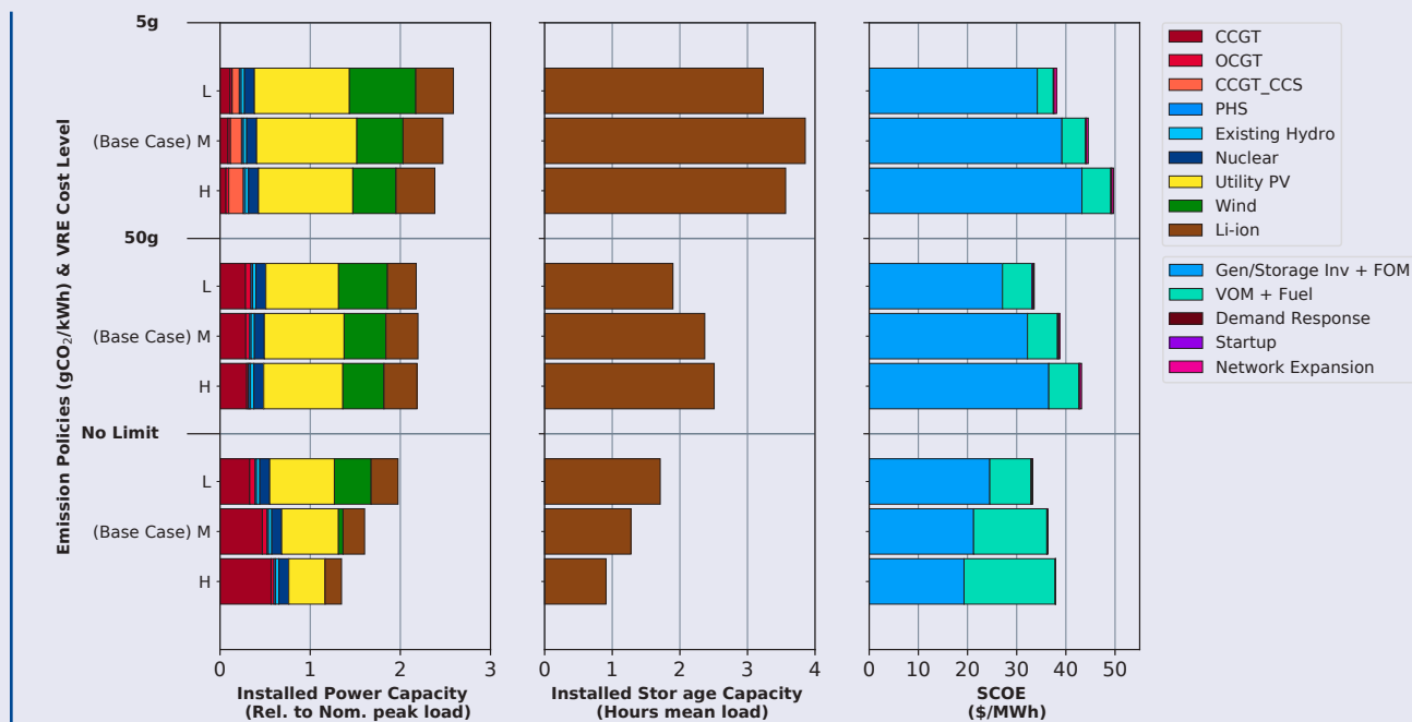
Figure C.10 System impacts of VRE at varying cost levels in the Southeast
