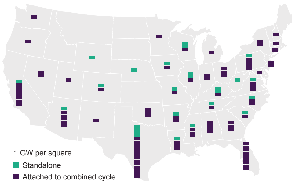
Figure 4.10 Geographic distribution of steam turbine capacity in the United States
