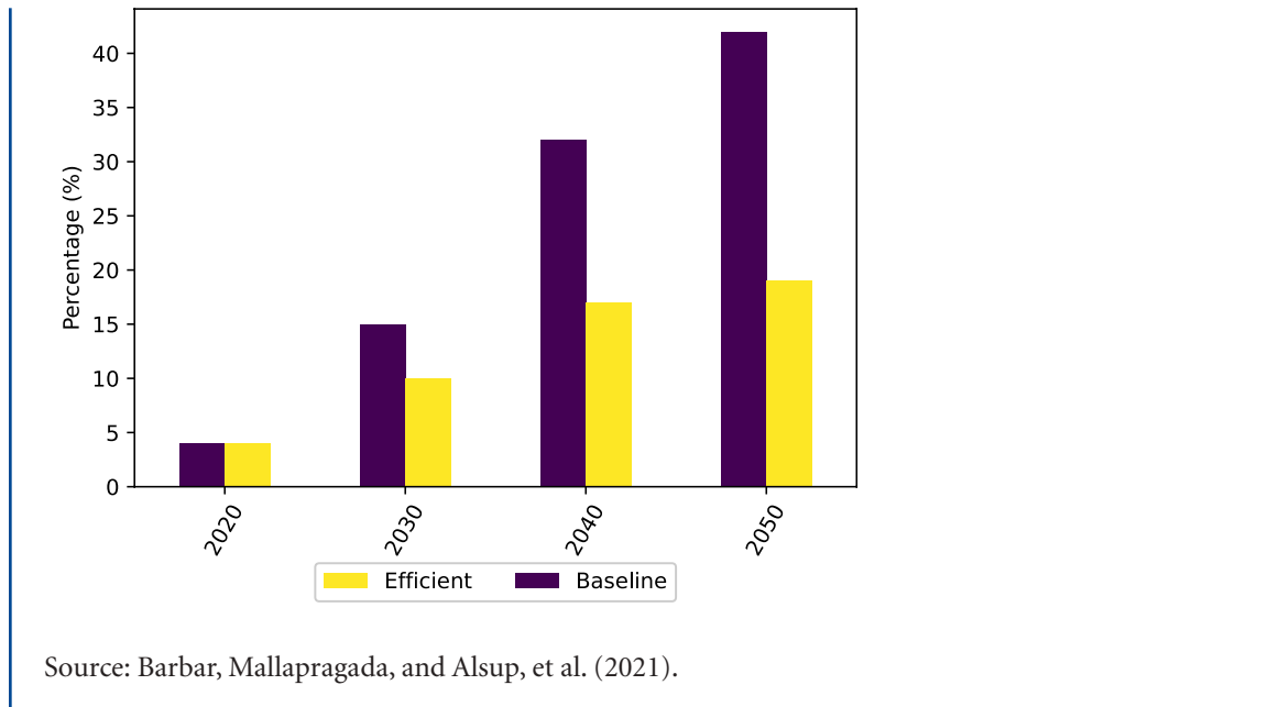
Figure 7.14 Cooling demand contribution to peak demand given space cooling demand growth, AC unit sales of various types, and average SEER projections for AC units sold in India
