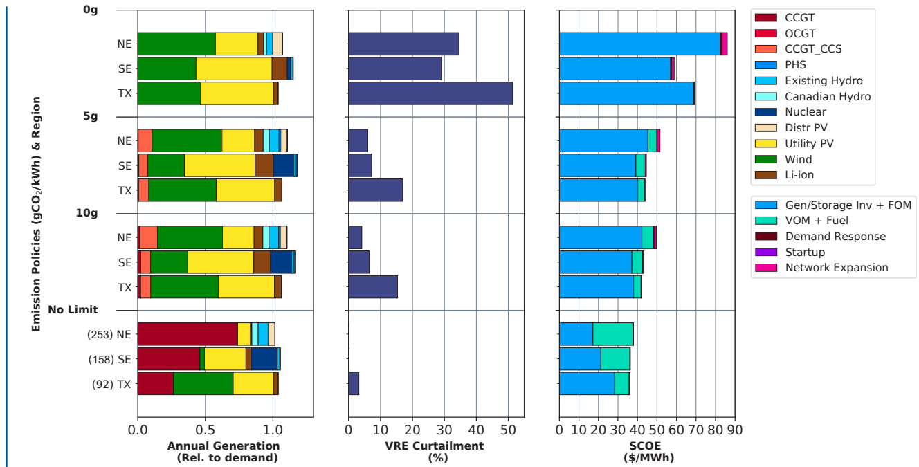
Figure 6.4 Annual generation, VRE curtailment, and system average cost of electricity (SCOE) in the Northeast (NE), Southeast (SE), and Texas (TX) under tightening CO 2 emissions constraints
