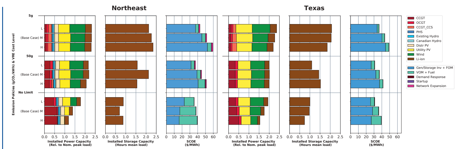
Figure 6.14 Impacts of low-, mid-, and high-cost VRE on installed power capacity, storage capacity, and SCOE across a range of CO 2 constraints for the Northeast and Texas regions
