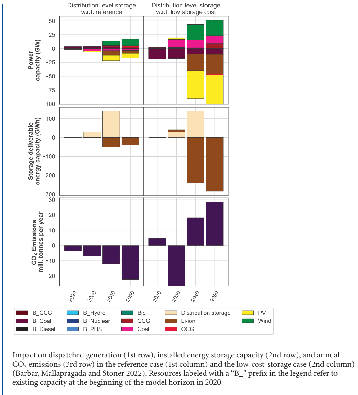
Figure 7.15 Distribution-level storage deployment
