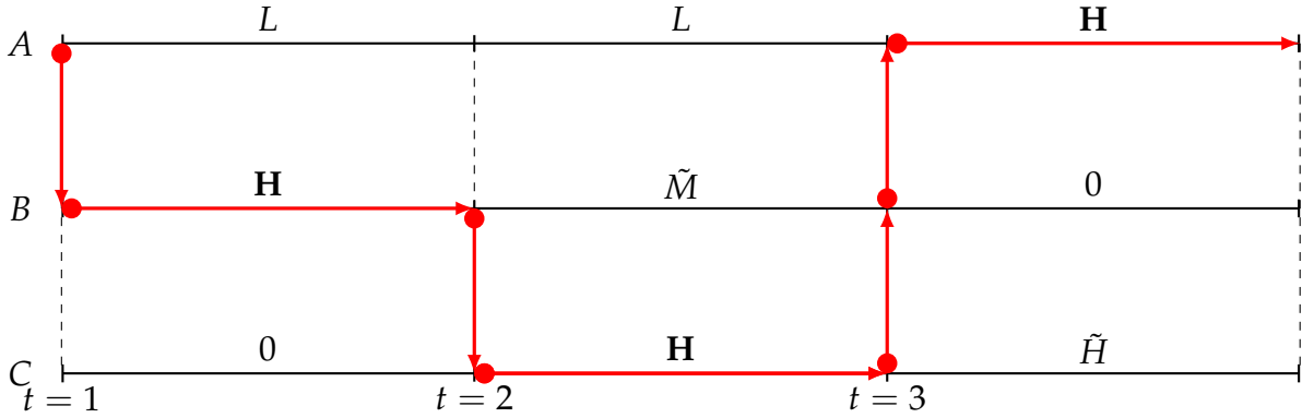
Figure 2: Optimal allocation of asset. This figure shows the optimal asset allocation between A , B , and C over t = 1, 2, 3 , which is achieved through two contracts: C_{AB}^{13} and C_{BC}^{23} . The red indicates ownership and transfer of the asset between traders. In the beginning of t = 1 , A starts with the asset, passes the asset to B , who holds it for one period. Then, B passes the asset to C , who holds it for one period to the end of t = 2 . At the beginning of t = 3 , the asset is transferred from C back to B to A , who holds it for the final period.
