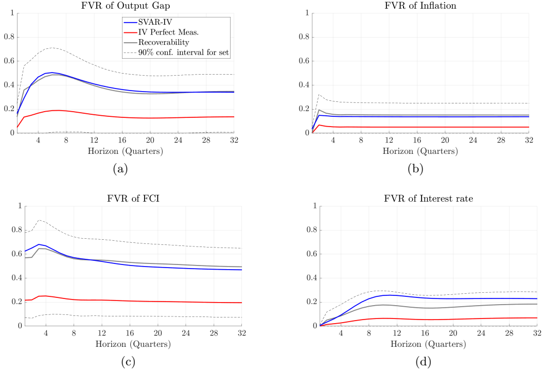
Figure 3: Identified Forecast Variance Ratios of the noise shock. Blue: SVAR-IV, assuming invertibility. Red: lower bound, assumes perfect measurement of the shocks. Grey: recoverability-based FVR. VAR includes the full set of macro outcomes (baseline + labor market variables). Dashed lines are 90% confidence intervals of the identified set, (Plagborg-Møller and Wolf, 2022) computed via bootstrap with 1000 repetitions.
