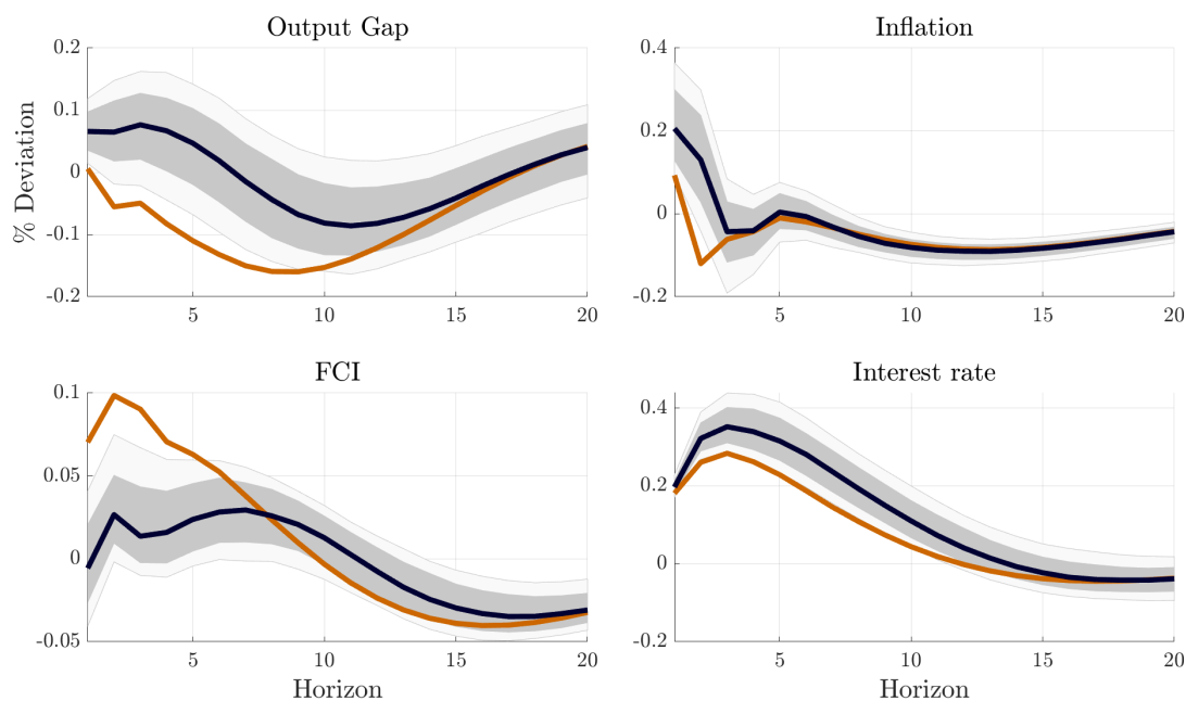
Figure 16: Counterfactual impulse response to a monetary policy shock, identified following Aruoba and Drechsel (2022). The orange line is the original point estimate, black line is the best approximation to the counterfactual impulse response. Shaded and light shaded grey bands indicate 68 and 90 confidence sets respectively.
