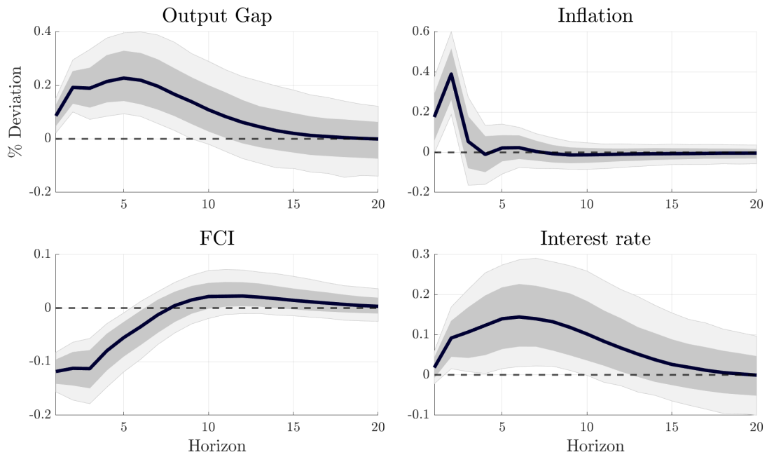
Figure 2: Impulse response to a financial noise shock. Shaded and light shaded grey bands indicate 68 and 90 confidence sets respectively.
