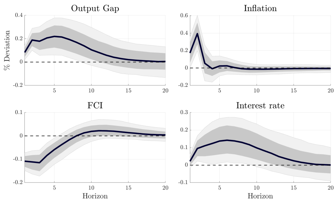
Figure 11: Impulse response to a financial noise shock, where the shock is identified controlling for 3 Principal Components in (B.2). Shaded and light shaded grey bands indicate 68 and 90 confidence sets respectively.
