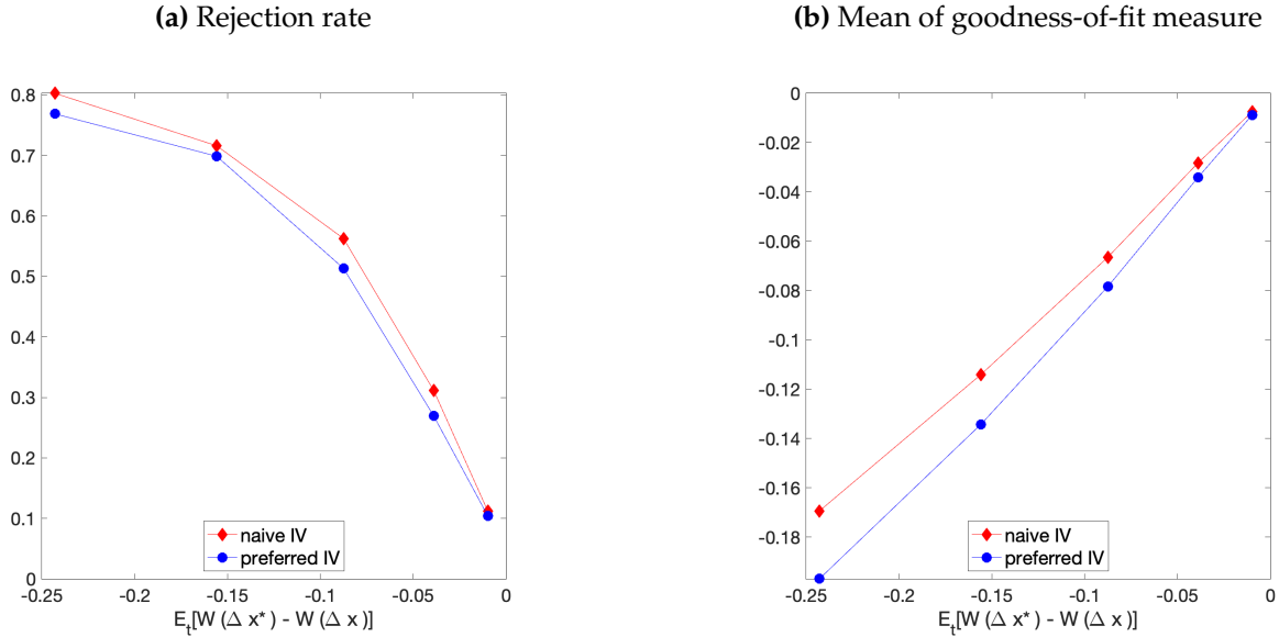
Figure B.3: Alternative IV-based Tests Under Misspecification from Linearization
