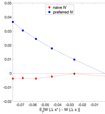
(b) Mean of goodness-of-fit measure ( \sigma_F )
