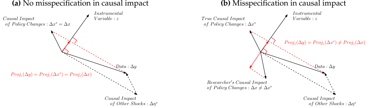
Figure 1: An IV-Based Measure of Goodness of fit
