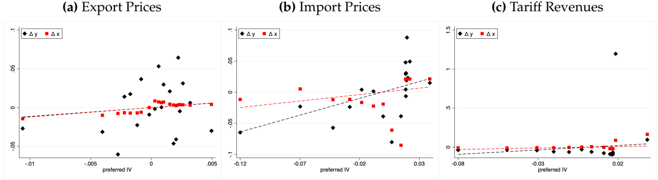
Figure 7: Observed versus Predicted Changes
