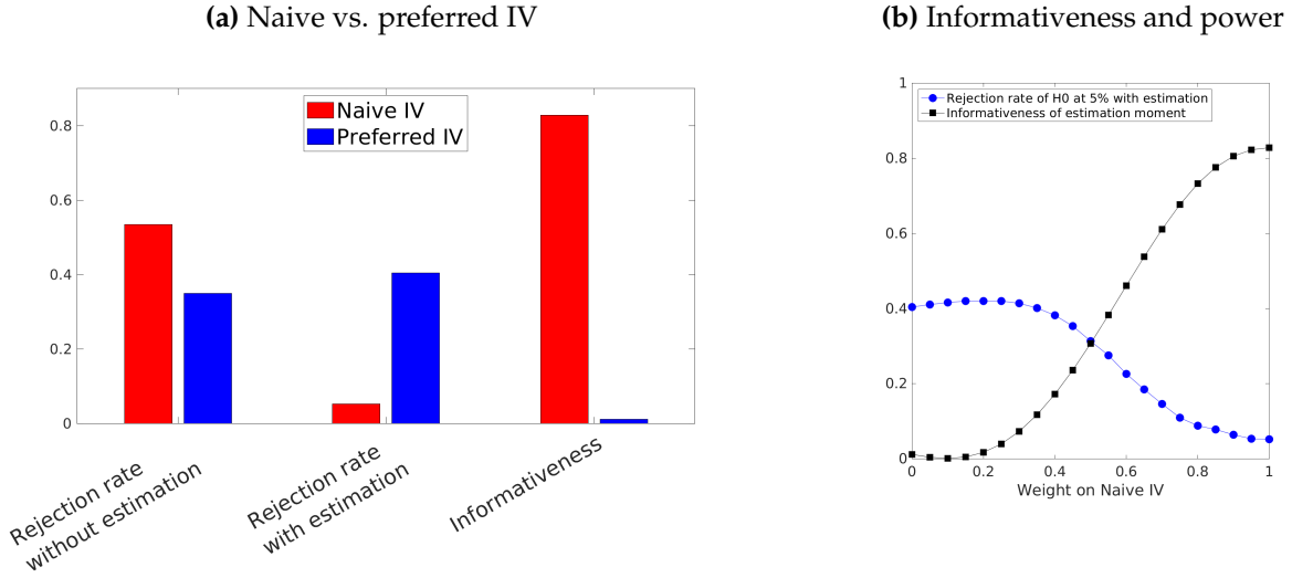
Figure 5: Estimation, Informativeness, and Mechanical Fit
