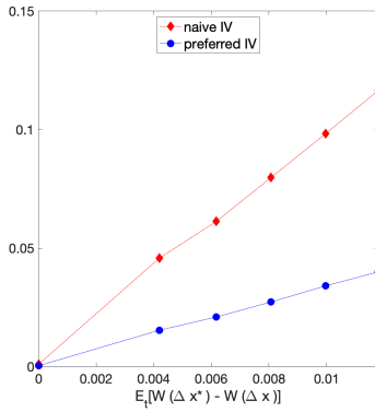
(a) Mean of goodness-of-fit measure ( \omega_F )
