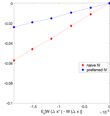
(c) Mean of goodness-of-fit measure ( \sigma )
