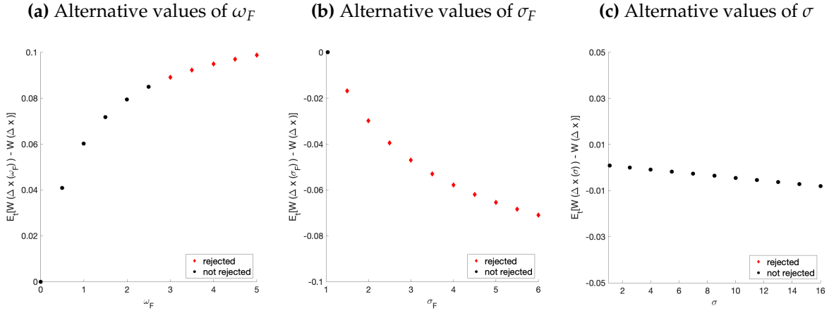
Figure 6: Welfare Predictions from Other Models
