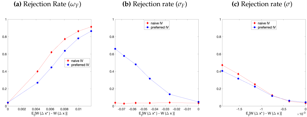
Figure 4: Alternative IV-based Tests with Incorrect Calibration
