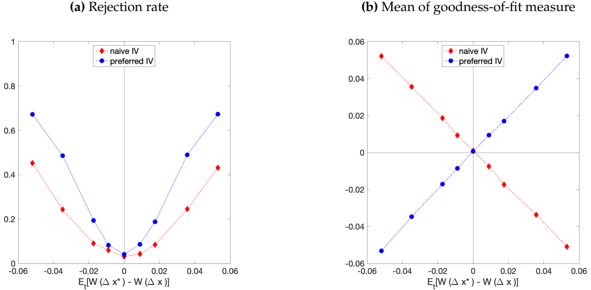
Figure 3: Alternative IV-based Tests Under Uniform Misspecification
