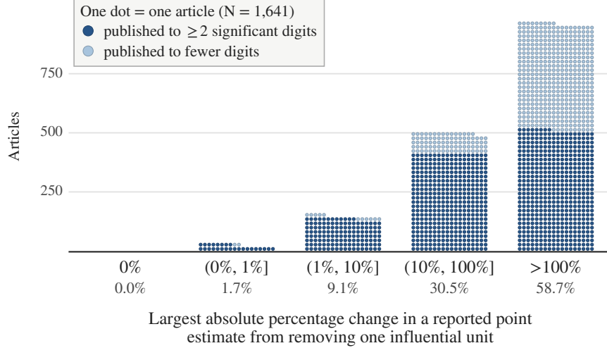
Figure 4: Sensitivity of reported estimates to removing an influential unit. Each dot represents one article; an article appears at most once, placed in the bin corresponding to the largest absolute percentage change, relative to our reproduction of the article’s reported value, among the point estimates we recalculated for that article after removing, one at a time, each of the 5 units with the largest influence on the point estimate under a linear approximation to the estimator, identified via the method of Giordano et al. (2026a,b). We conducted this sensitivity analysis for the 1,908 articles in which there is at least one reproducible point estimate whose associated inferential method suggests the existence of an independent unit (e.g., observation or cluster) and for which we could reconstruct the empirical influence function. The plot excludes articles where the largest absolute percentage change is for a point estimate whose published value is zero at printed precision. Dark dots correspond to results whose published value is printed to at least two significant digits; light dots to results printed with fewer. Percents need not add to 100 due to rounding.
