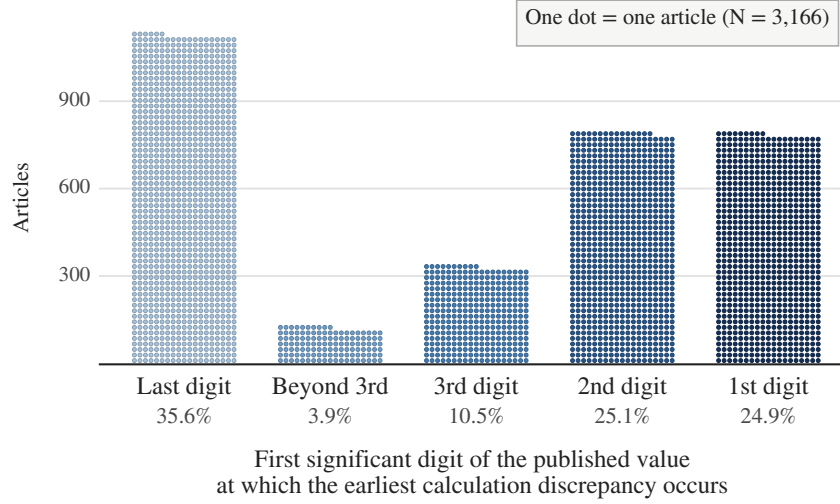
Figure 3: Significant digit of earliest calculation discrepancy. Each dot represents one article whose earliest discrepancy is a calculation that we recompute at a different value from the published one; an article appears at most once. “Last digit” collects articles whose recomputed value agrees with the published value to within 1.0 units of the last printed digit, as might be consistent with rounding or truncation. The remaining articles are placed in the bin corresponding to the earliest significant digit of the published value at which the recomputed value, rounded to the published precision, differs. The “beyond 3rd” category includes differences past the third significant digit. The “1st digit” category includes differences at or before the published value’s first significant digit. The plot excludes articles where the earliest discrepancy is for a calculation that is not printed as a number (e.g., reported as a range). Percents need not add to 100 due to rounding.
