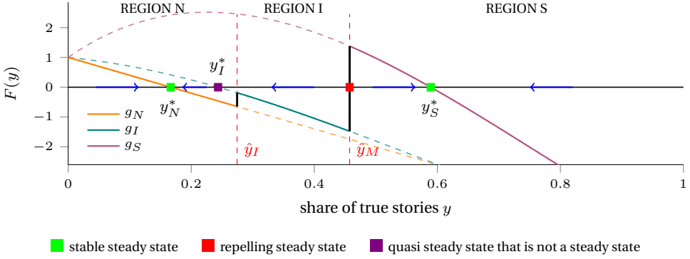
FIGURE 1. The LDI for \rho = 40 , \kappa = 5 , \theta = 0.9 , \mu = 2.6 , \beta = 1 , \delta = 0.65 , \lambda = 0.9 . Within each region the LDI is single-valued and coincides with the regional drift g_R (solid); the dashed curves continue each g_R outside its region. At the thresholds the LDI is set-valued, shown by the black segments.
