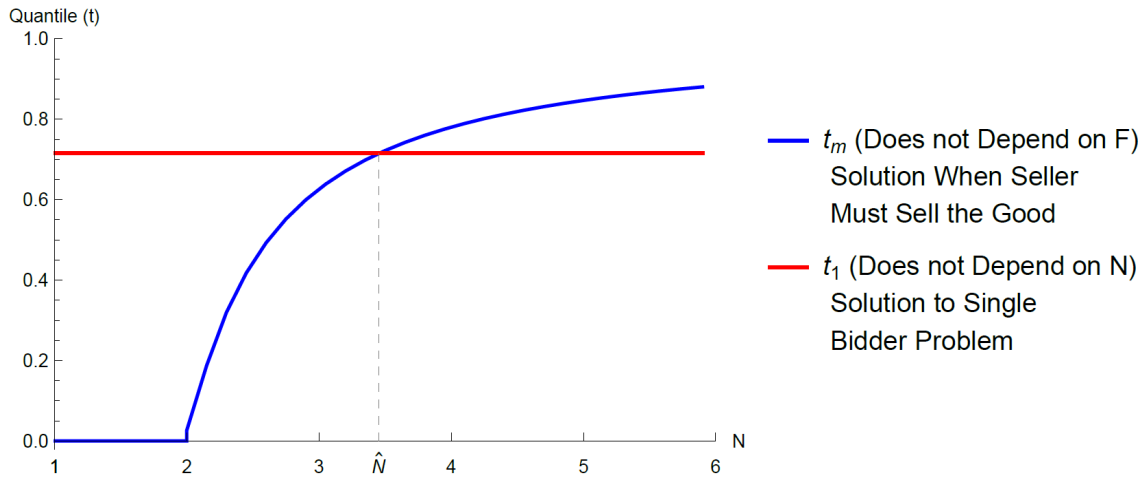
Figure 11: Threshold Values of the Solution to the Restricted Problems: (i) N=1 and (ii) Must Sell Mechanism.
