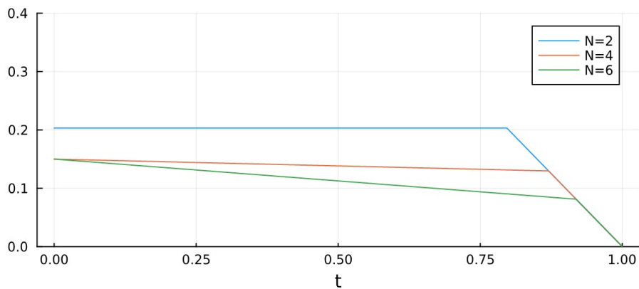
Figure 5: Revenue Function \pi(t|t_z) with m = 0.15 .
