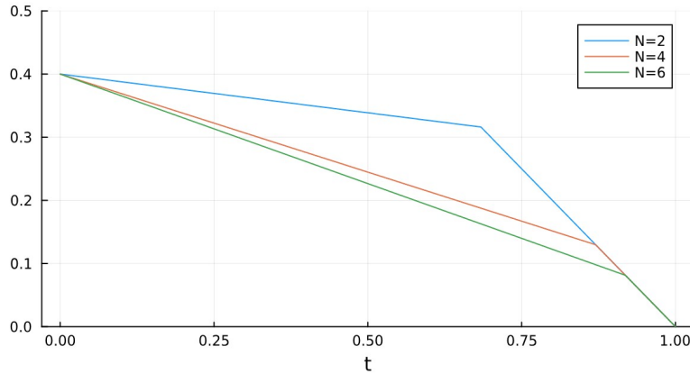
Figure 7: Revenue Function \pi(t|t_z) with m = 0.4 .
