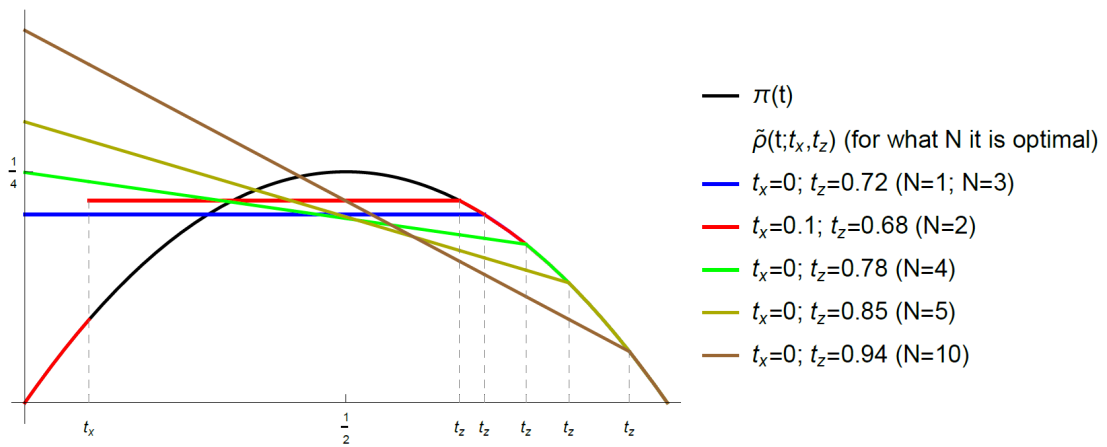
Figure 10: Revenue Functions in Quantile Space for Uniform Distribution F(v) = v .
