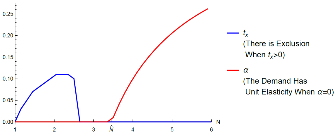
Figure 12: Solution to General Problem with N > 1
