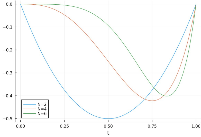
Figure 1: Probability Differential of First and Second Order Statistic
