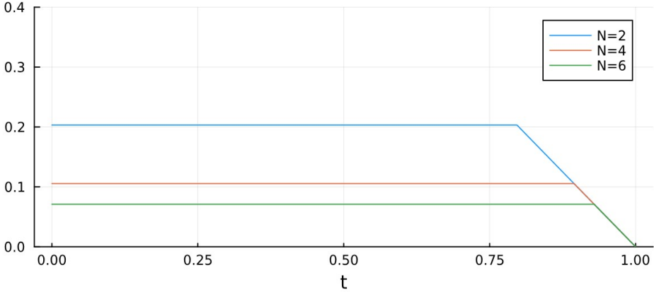
Figure 3: Revenue Function \pi(t|t_z) with m = 0 .
