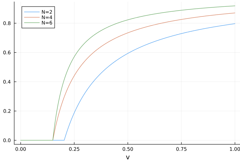
Figure 4: Distribution Function G(t|t_z) with m = 0.15 .
