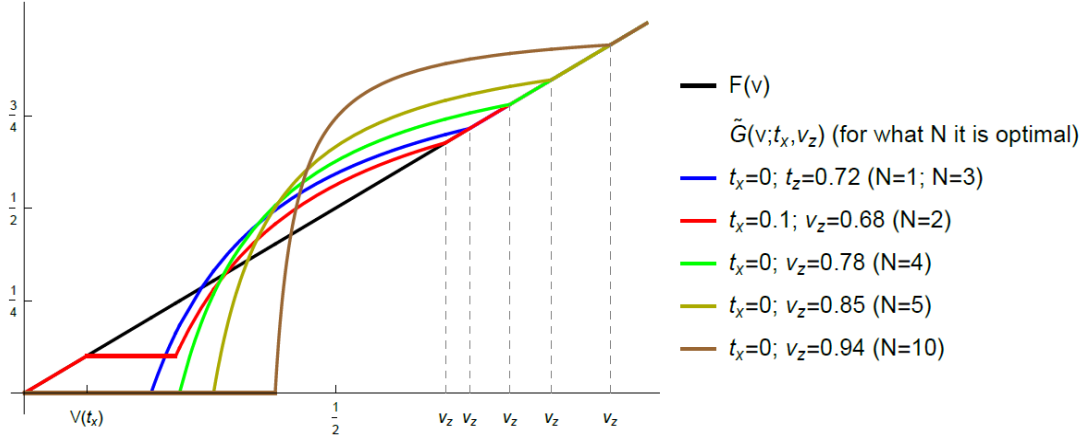
Figure 8: Prior and Posterior Distributions in Value Space v, w
