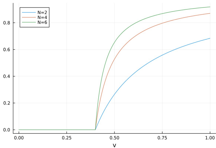
Figure 6: Distribution Function G(t|t_z) with m = 0.4 .
