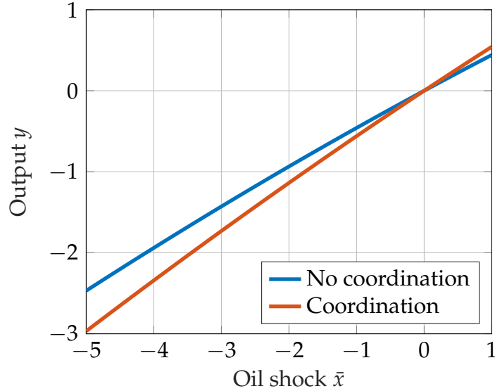
Figure 4: Comparative statics
