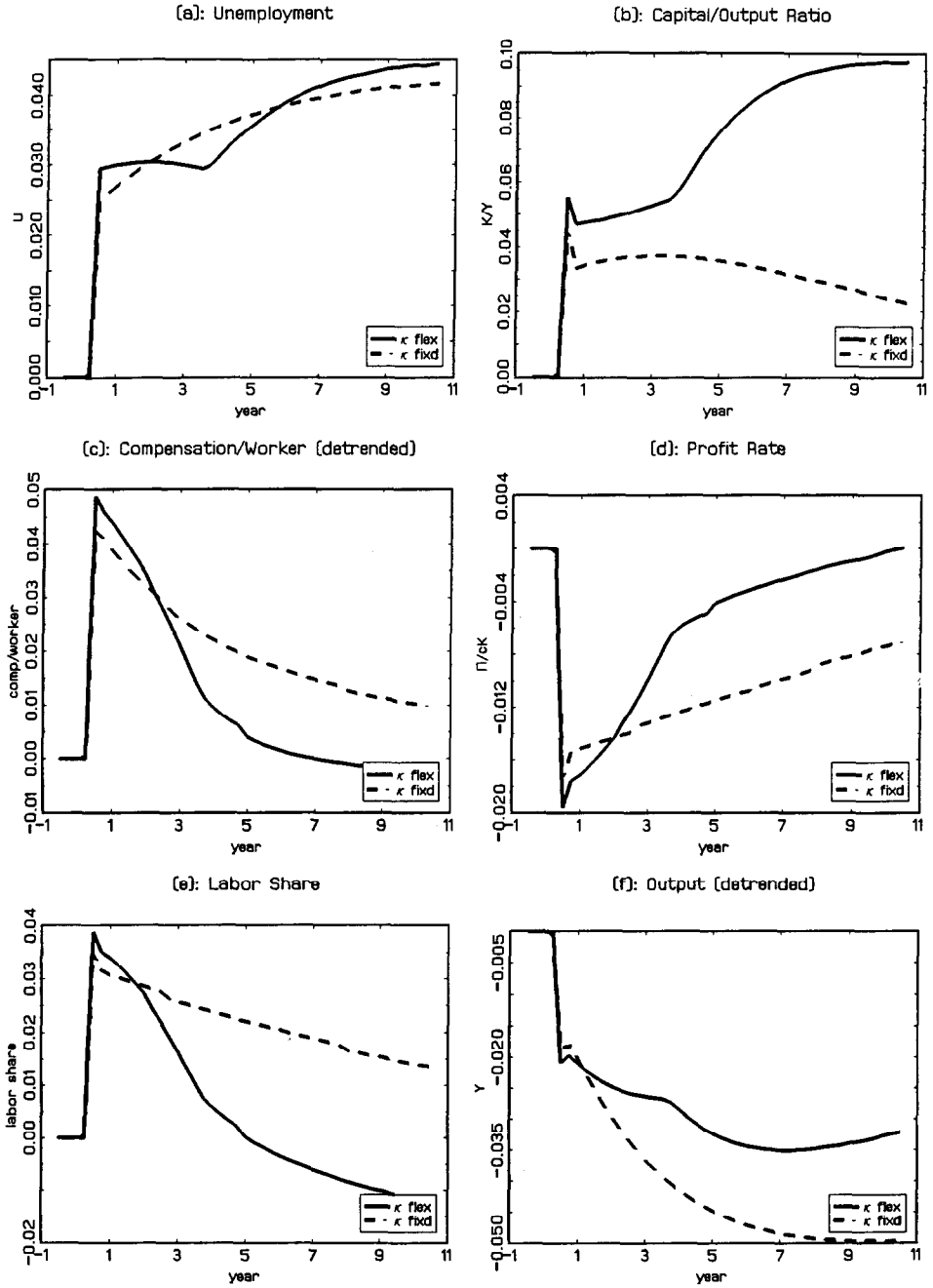
Figure 4.2 : Response to an Appropriation Shock
