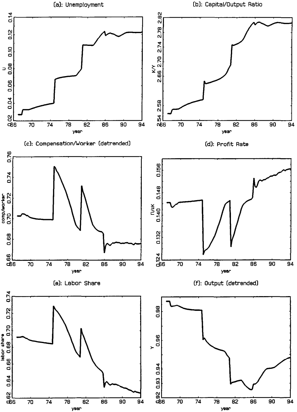
Figure 4.3 : Simulation Based on France
