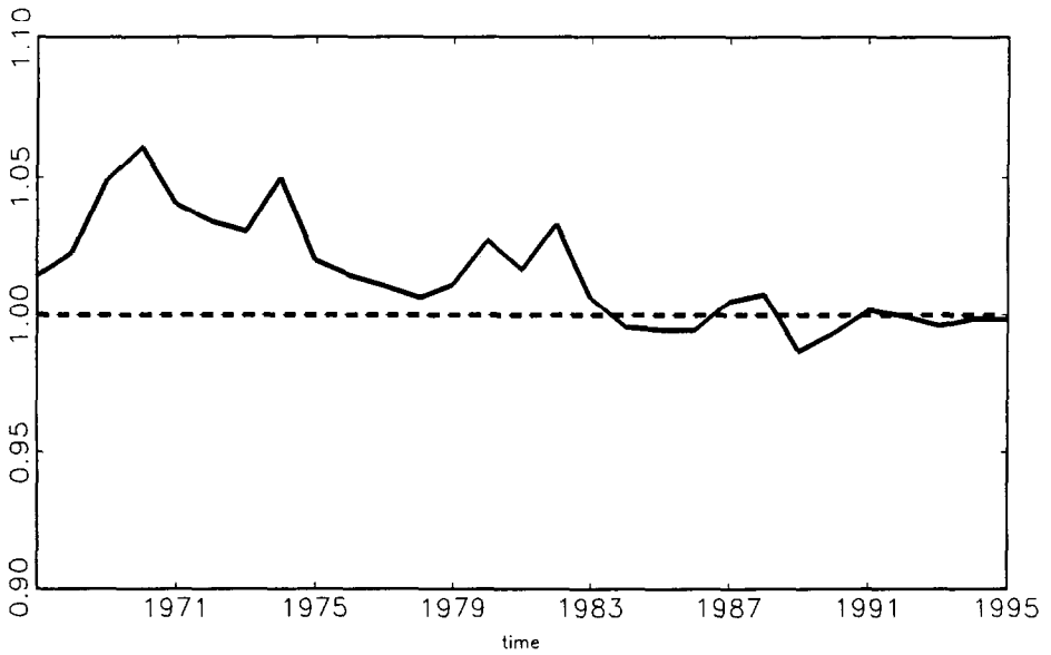
(b): US; Wage over Y_L (Cobb-Douglas)
